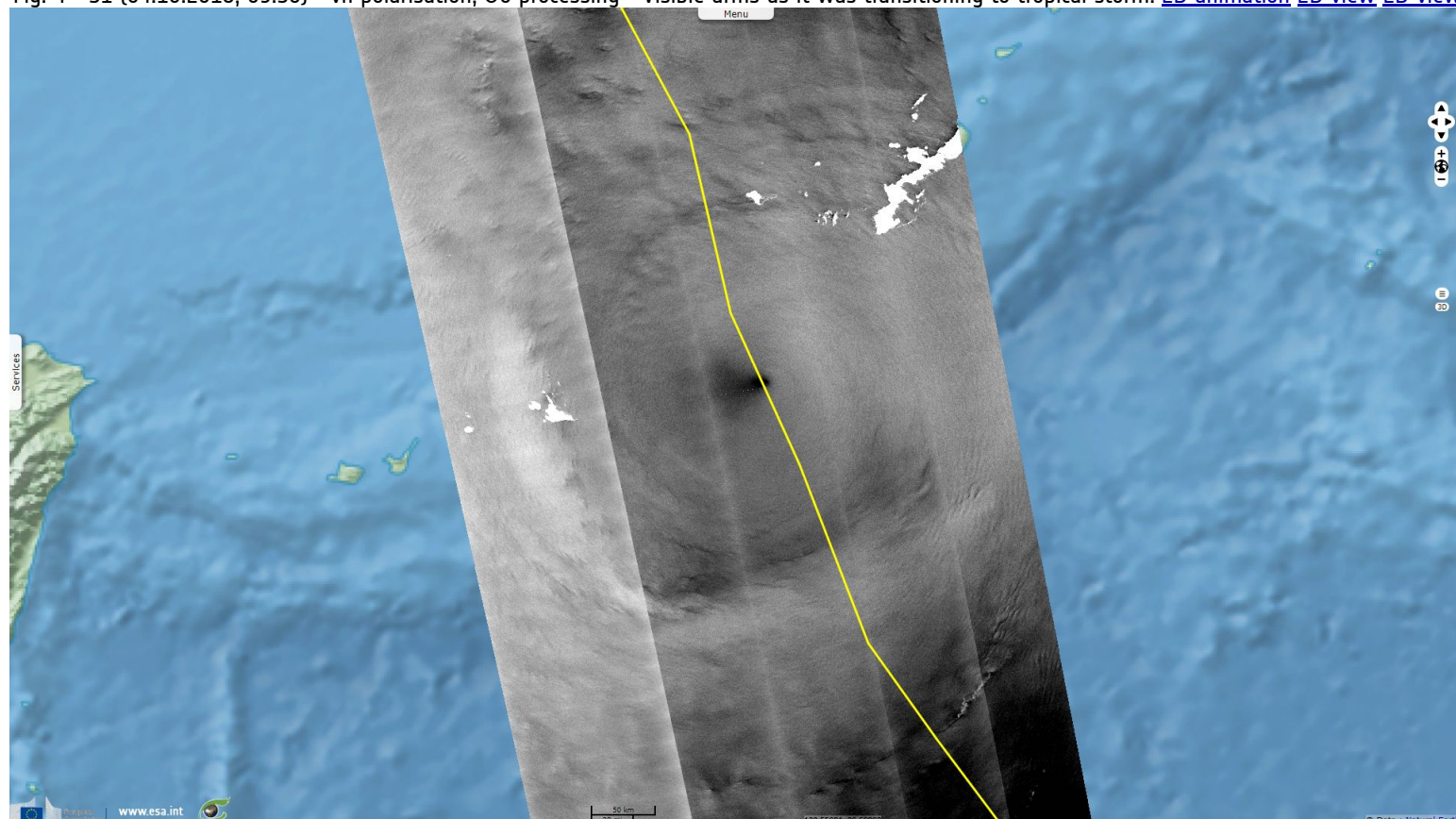
Fig. 4 - S1 (04.10.2018, 09:36) - vh polarisation, \sigma_0 processing - Visible arms as it was transitioning to tropical storm. 2D animation 2D view 2D view
