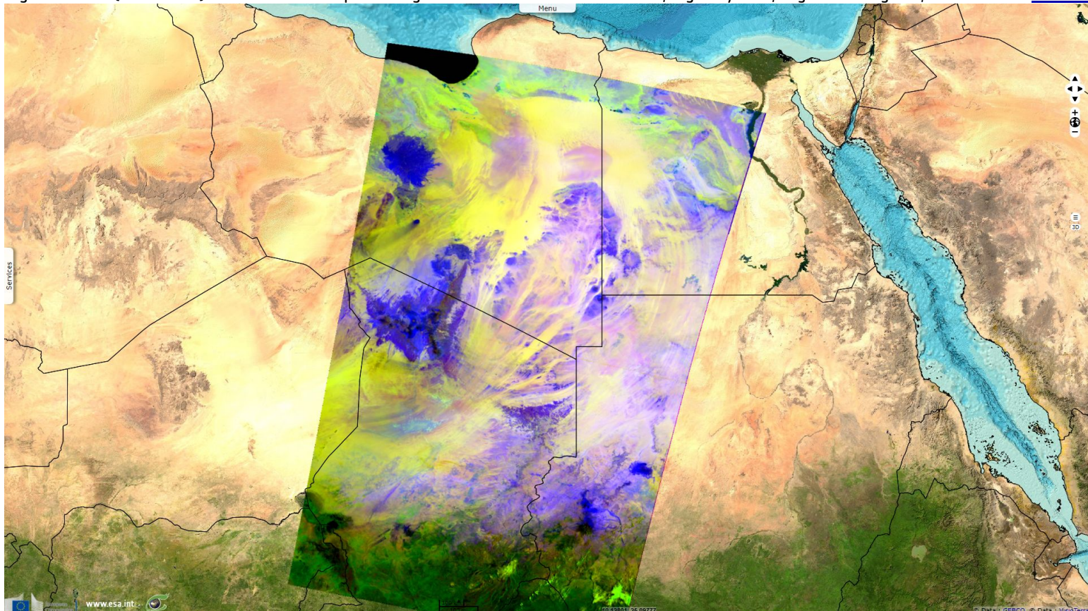
Fig. 2 - OLCI - 10-6-3 natural colour - Granitic intrusions surrounded by red sands around Gilf el-Kebir region. 2D animation 2D view 3D view
