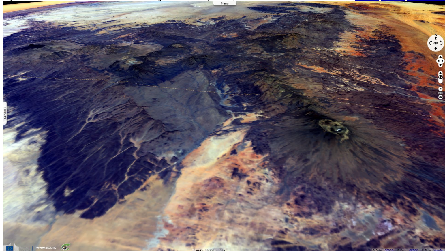
Fig. 4 - SLSTR (07.03.2017) - 6-3-1 colour composite - Wind shaped landscape between Tiberti range and Ennedi plateau.
