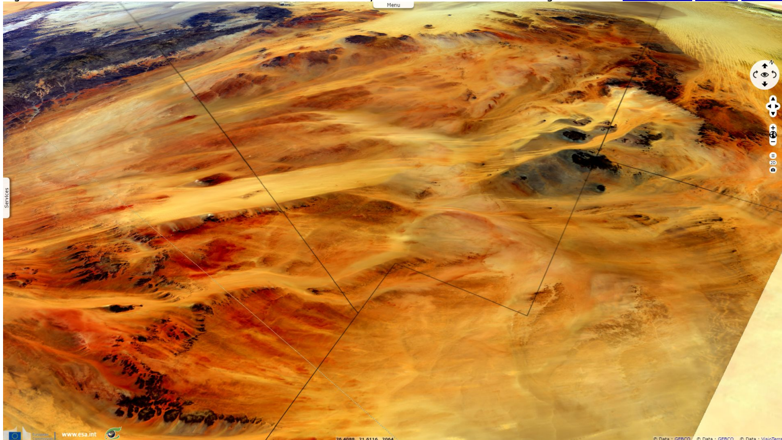
Fig. 2 - OLCI - 10-6-3 natural colour - Granitic intrusions surrounded by red sands around Gilf el-Kebir region. 2D animation 2D view 3D view
