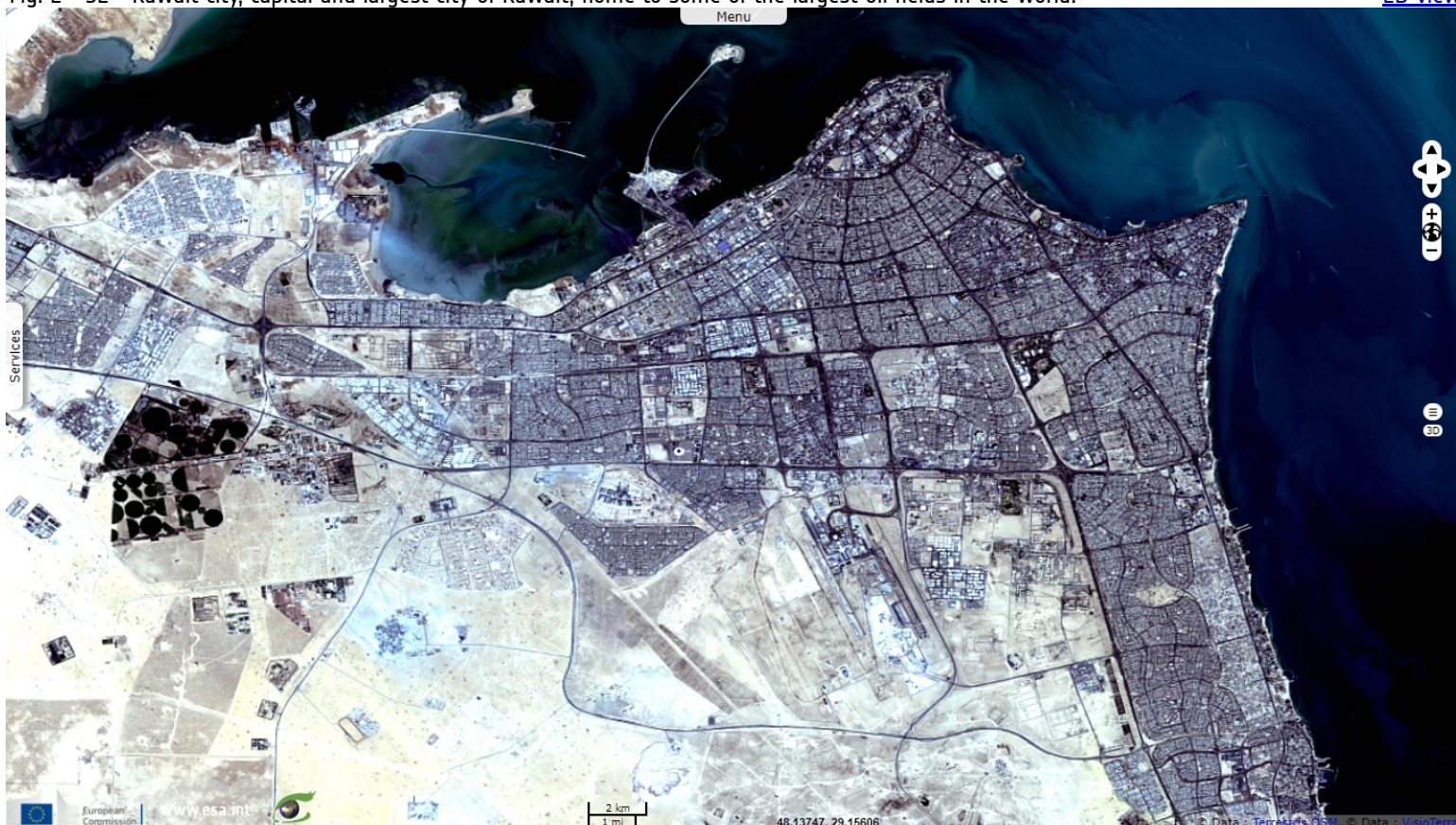
Fig. 2 - S2 - Kuwait city, capital and largest city of Kuwait, home to some of the largest oil fields in the world.
