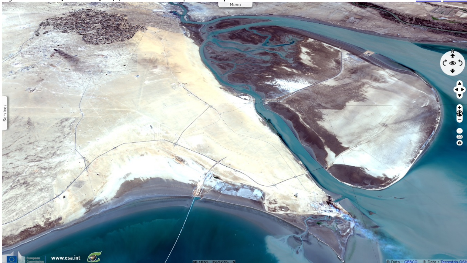
Fig. 1 - Sentinel 2 (2018-02-05) - 4,3,2 natural colour composite - Bubiyan island & Sabah Al-Ahmad Natural Reserve.
