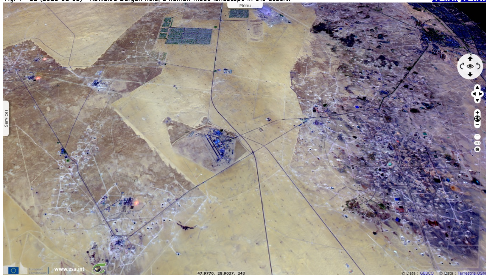
Fig. 4 - S2 (2018-02-05) - Kuwait's Burgan field, a human-made landscape in the desert.
