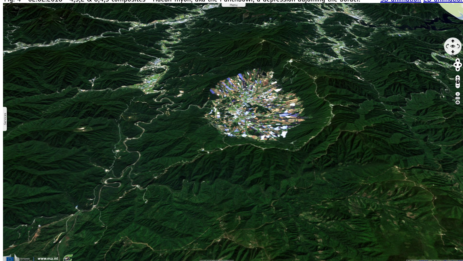
Fig. 4 - 02.02.2018 - 4,3,2 & 8,4,3 composites - Haean-myon, aka the Punchbowl, a depression adjoining the border.
