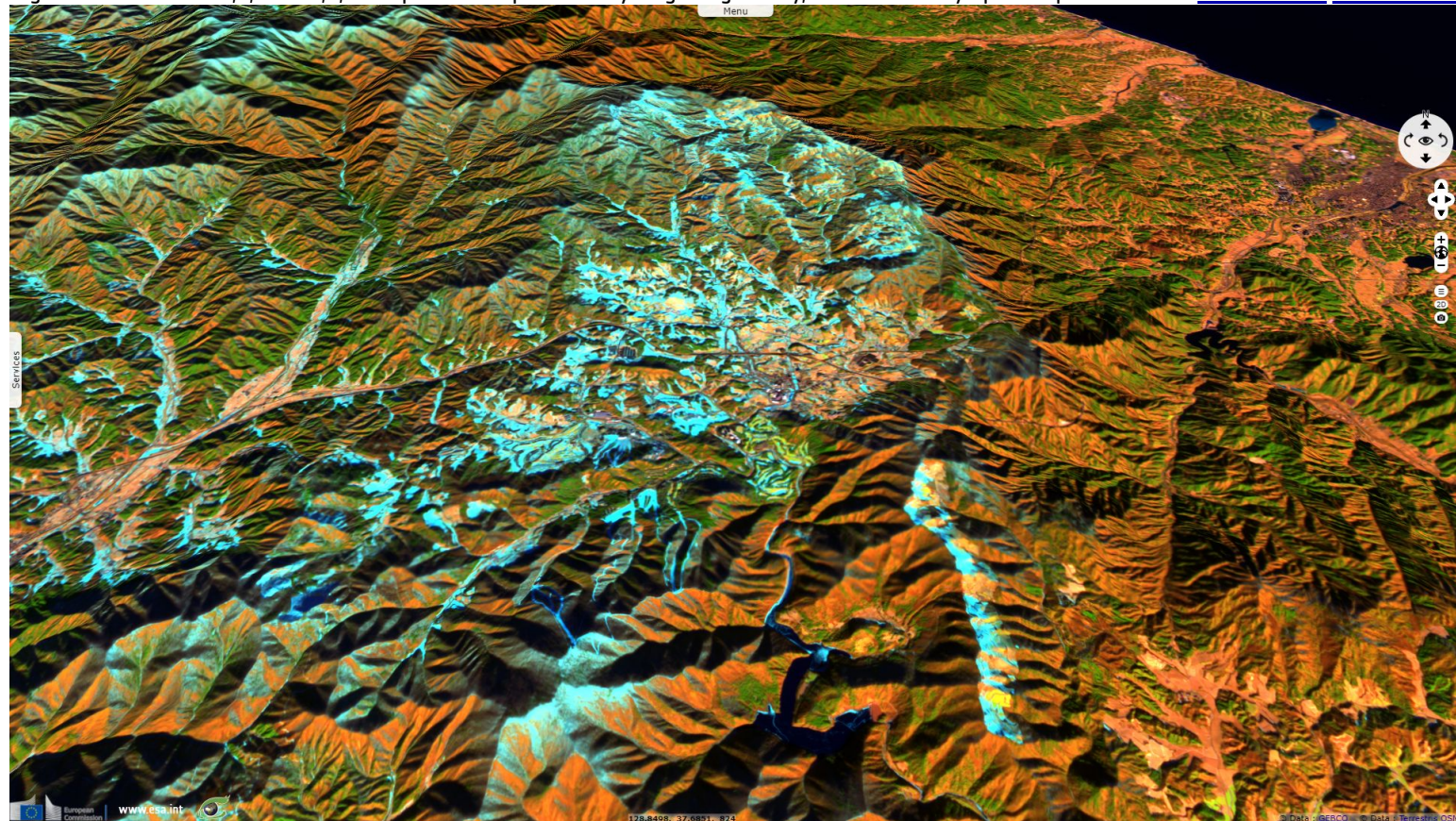
Fig. 5 - 21.12.2017 - 8,4,3 & 11,8,2 composites - Alpensia in Pyeongchang county, heart of the Olympic competition.
