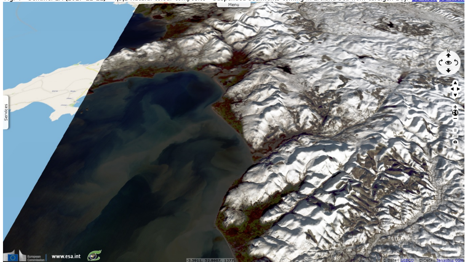
Fig. 4 - Sentinel 2A (2017-12-11) - 4,3,2 Natural colour composite - Suspended sediments coming in Ireland Sea from Cardigan Bay. 2D view 3D view
