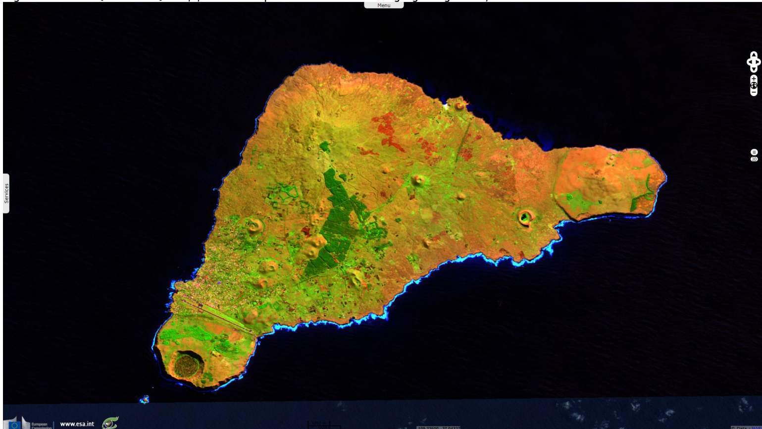
Fig. 2 - Sentinel-2 (26.07.2017) - 12,8,2 colour composite - Infrared bands highlight vegetation, bare soils and old lava flows.
