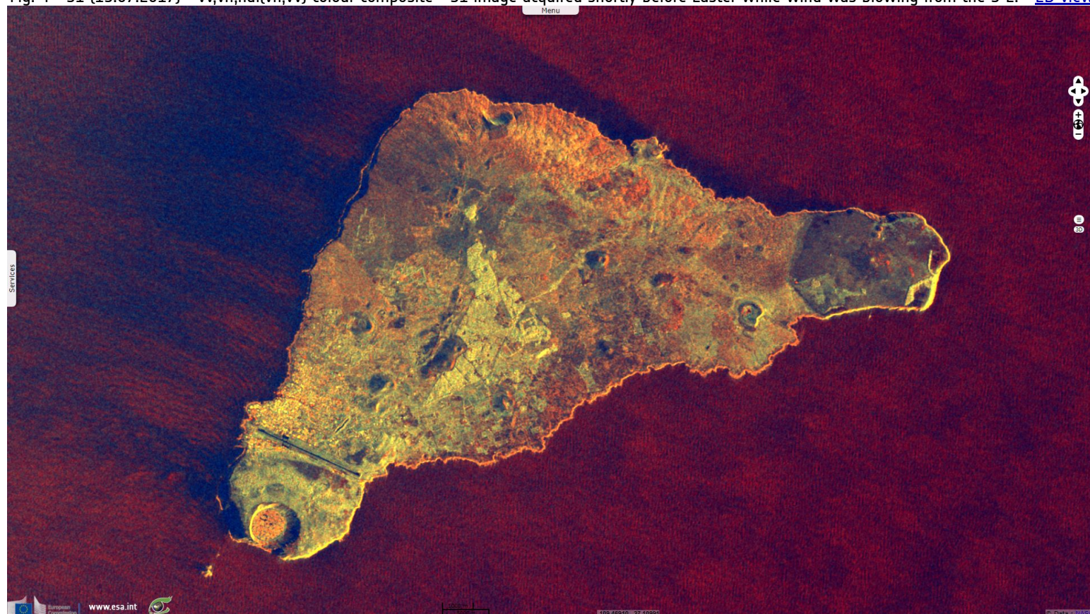
Fig. 4 - S1 (13.07.2017) - vv,vh,ndi(vh,vv) colour composite - S1 image acquired shortly before Easter while wind was blowing from the S-E.
