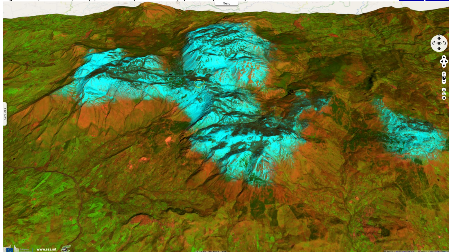
Fig. 4 - S2 (25.10.2018) - 4,3,2 natural colour - The first of the 4-nodes network will be built on 1865m high Monte Mufara. 3D view 2D view
