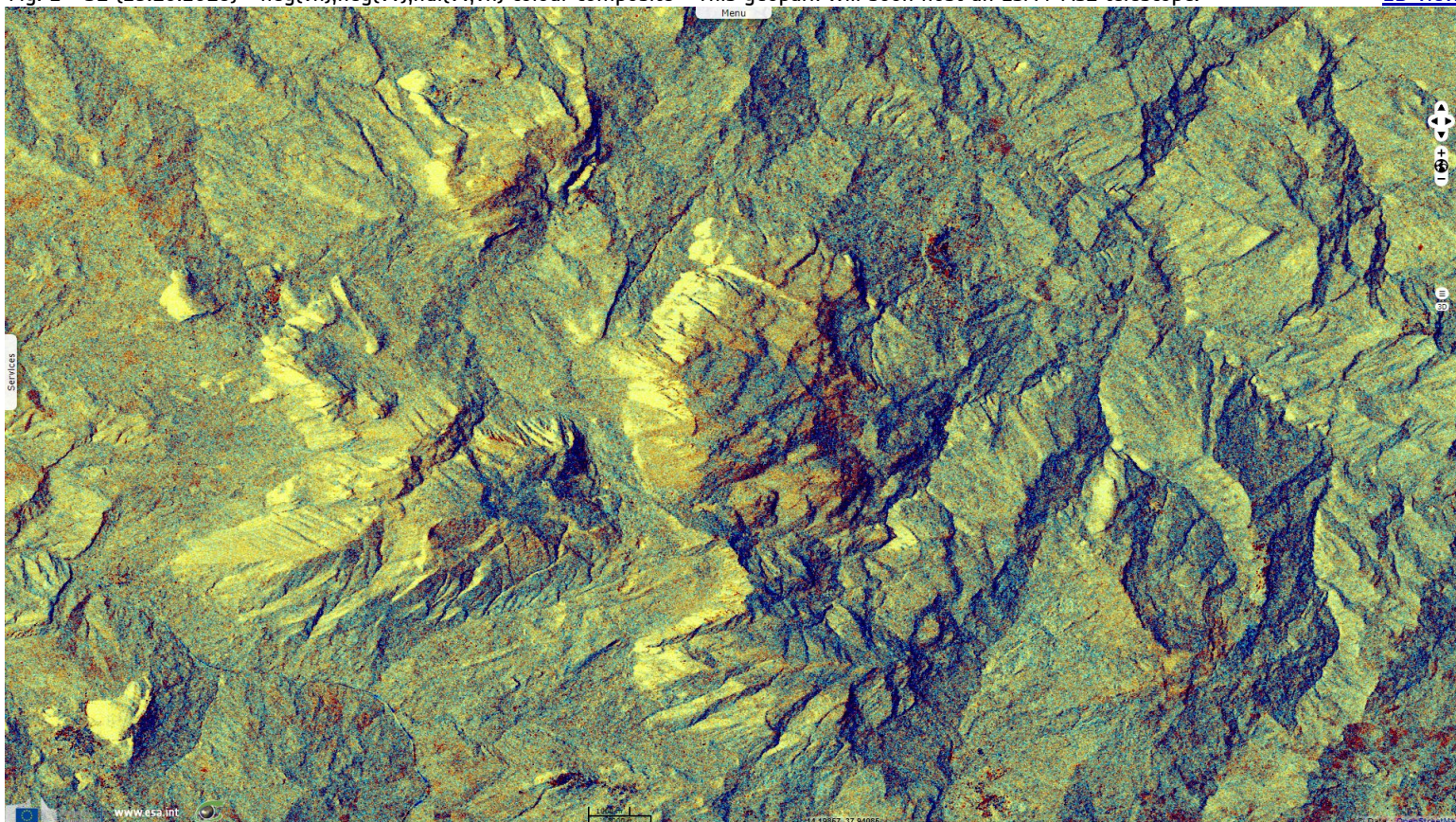
Fig. 2 - S1 (29.10.2018) - \text{neg(vh)}, \text{neg(vv)}, \text{ndi(vv,vh)} colour composite - This geopark will soon host an ESA / ASI telescope.
