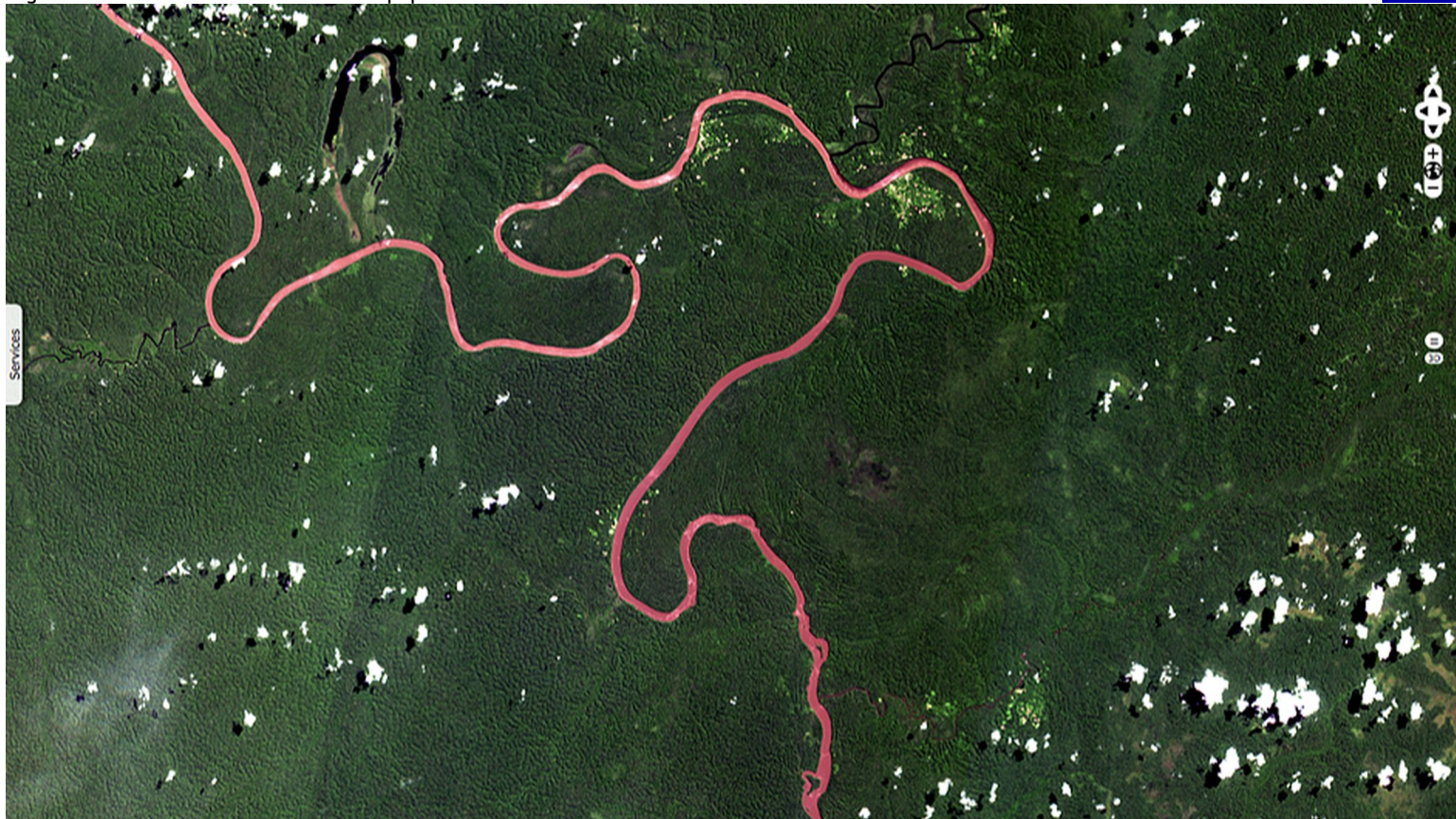
Fig. 2 - S2A MSI - Red colours in Río Apaporis.
