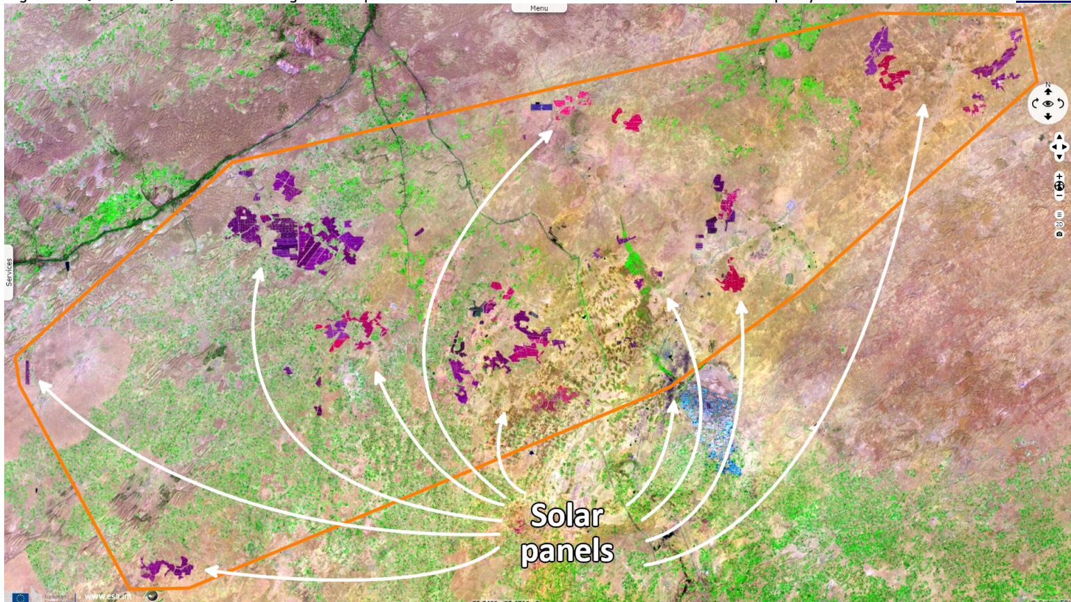
Fig. 2 - S2 (11.03.2023) - This is the largest solar park in the World with a surface of 5700 ha and a total capacity of 2245 MW. 3D view
