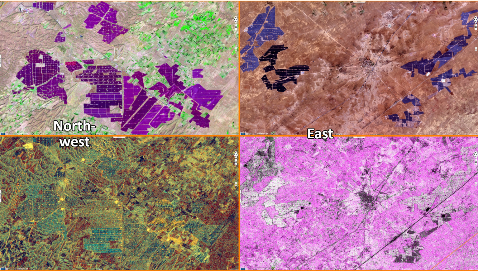
Fig. 3 - S2 (11.03.2023) / S1 (04.02.2023->12.03.2023) - Normal temperatures in Bhadla hover around 46-48 °C, with hot winds and sand storms occurring frequently.
