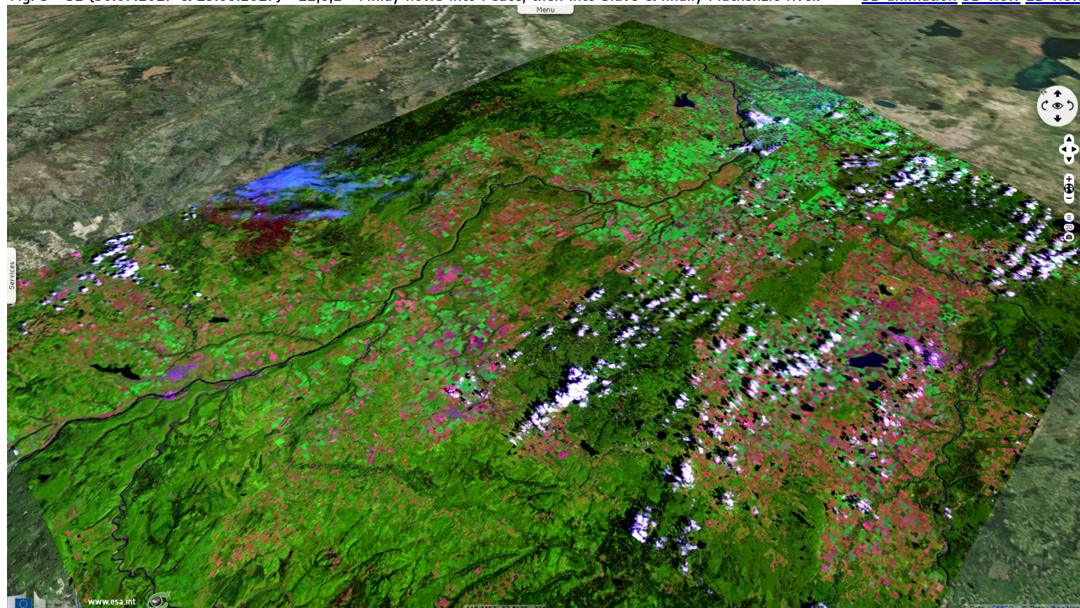
Fig. 4 - S2 (26.04.2018) - 12,8,2 composite - It reaches the Arctic Ocean via the Beaufort Sea after a 4241 km course.
