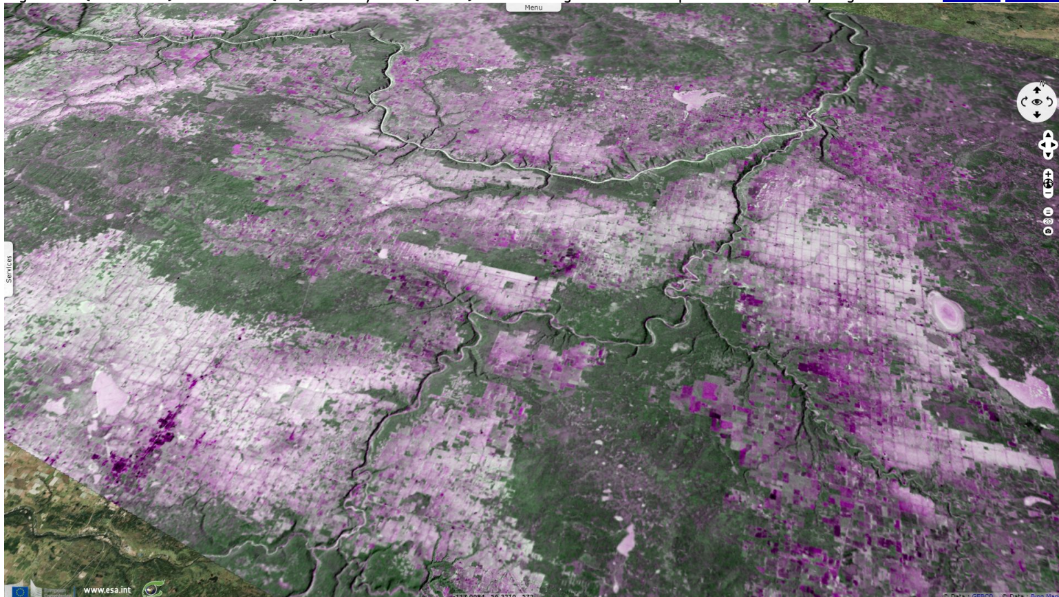
Fig. 2 - S1 (25.04.2018) - Peace river (left) & Smoky river (bottom) cleave through the Albertan plateau before they merge.
