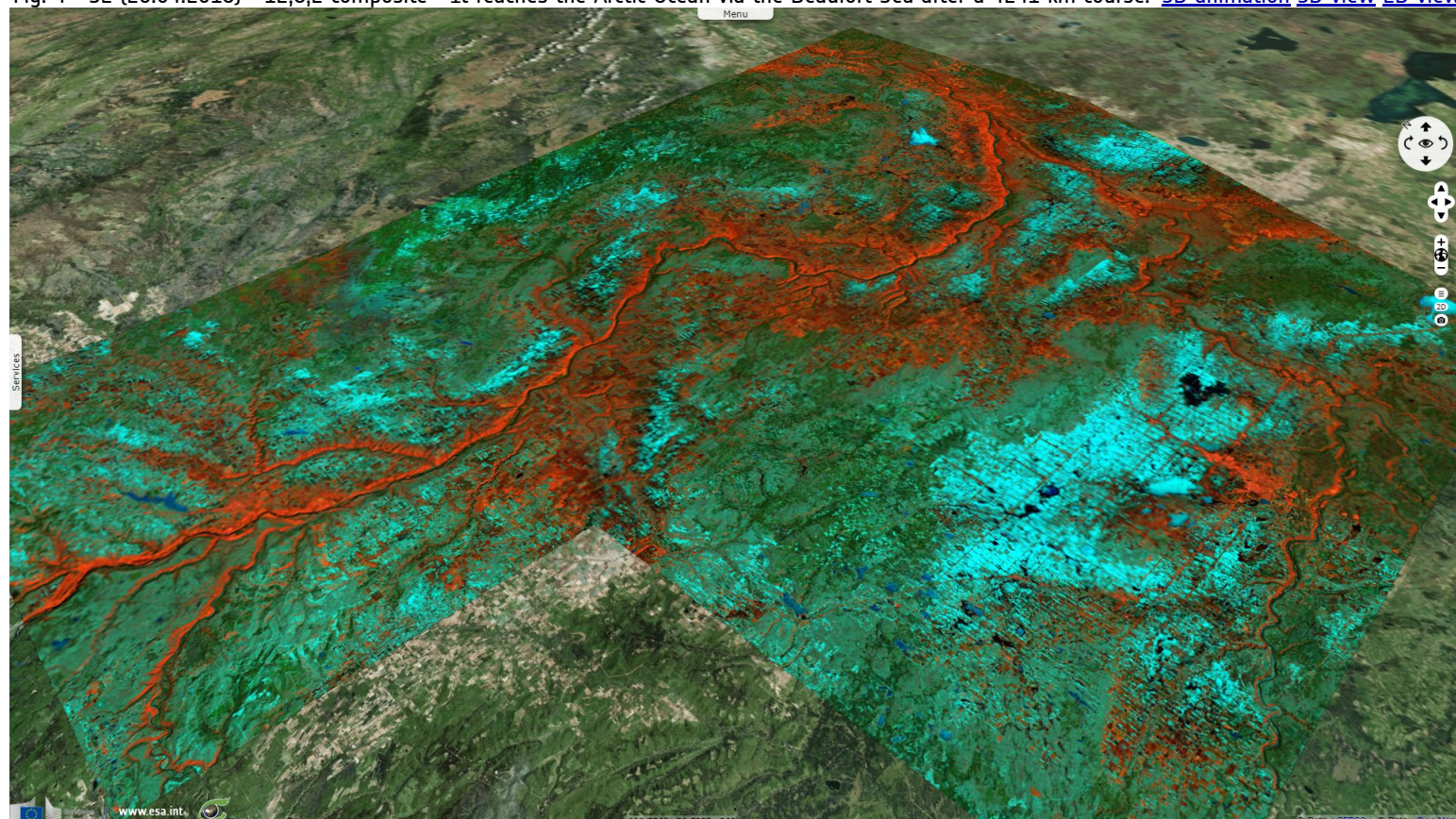
Fig. 4 - S2 (26.04.2018) - 12,8,2 composite - It reaches the Arctic Ocean via the Beaufort Sea after a 4241 km course.
