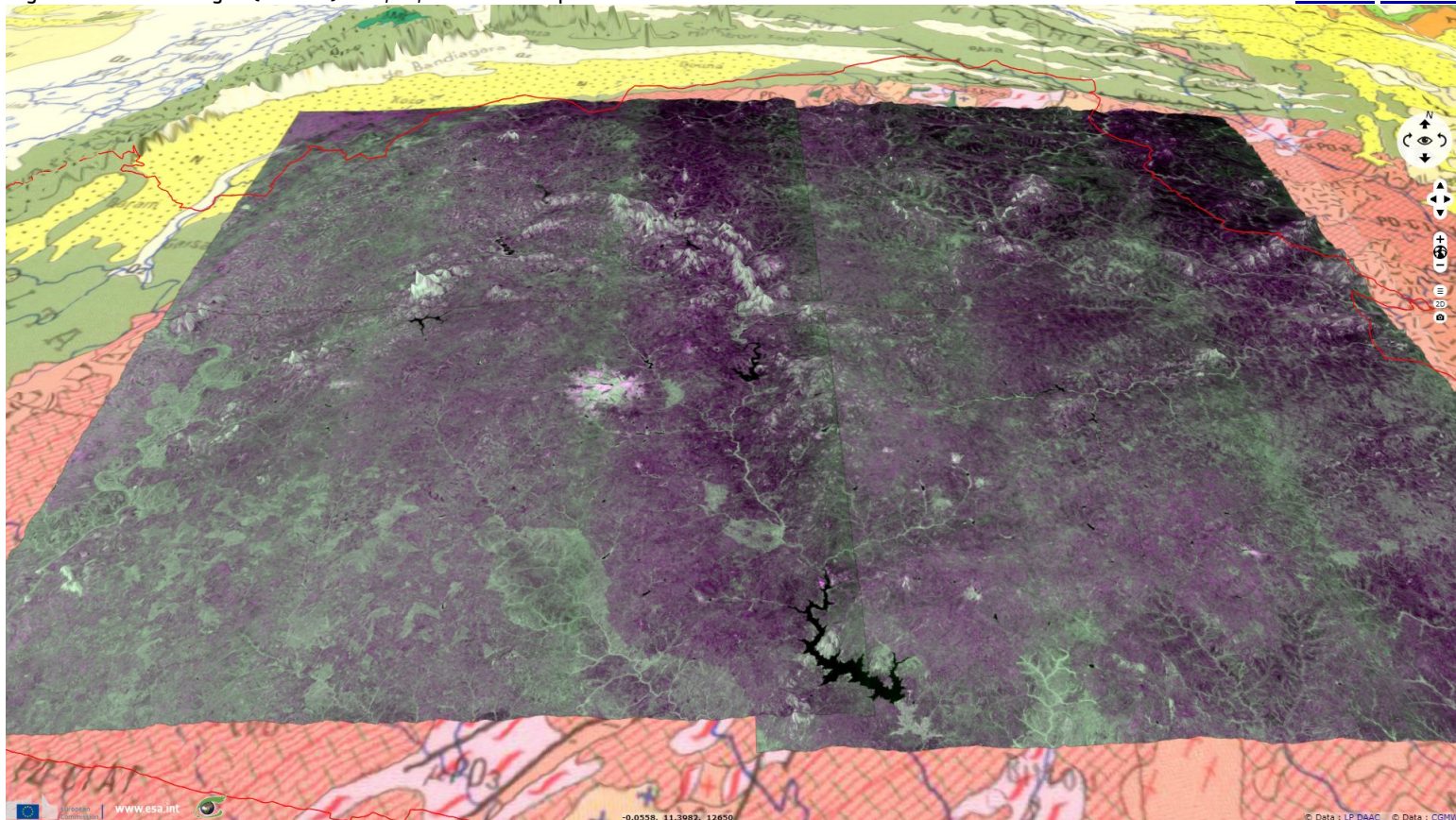
Fig. 2 - S1 mean images (4 dates) - VV,VH,VV colour composite - View of the east of Burkina Faso.
