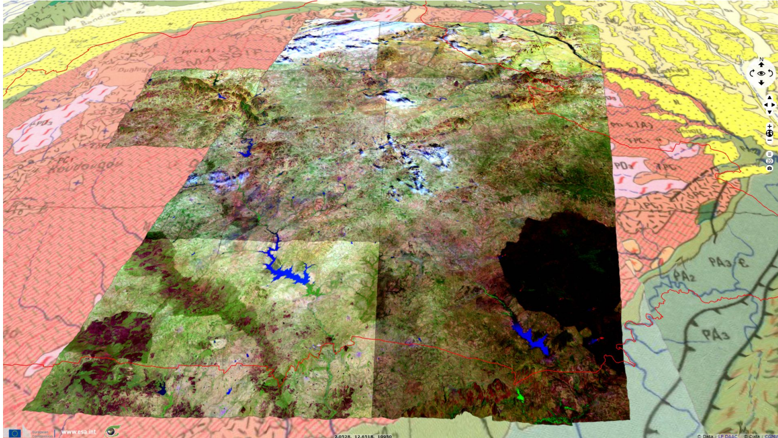
Fig. 2 - S1 mean images (4 dates) - VV,VH,VV colour composite - View of the east of Burkina Faso.
