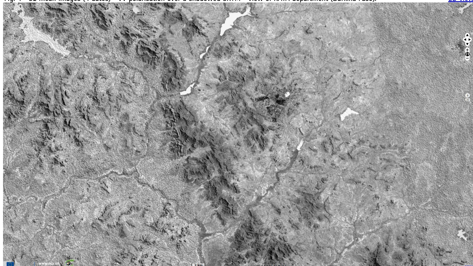
Fig. 4 - S1 mean images (4 dates) - VV polarisation over a shadowed SRTM - View of KAYA department (Burkina Faso).
