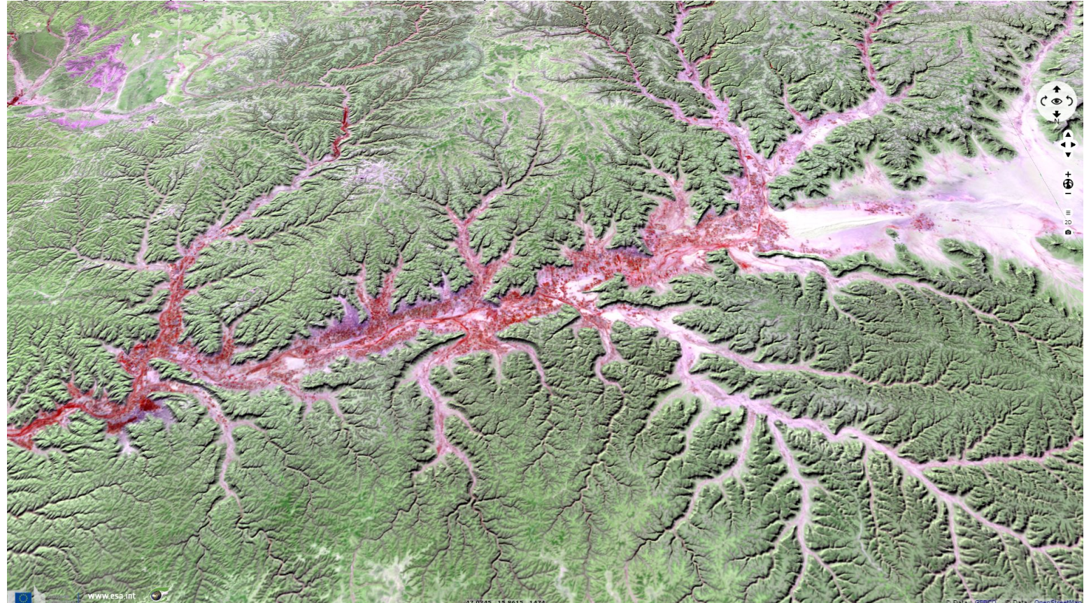
Fig. 4 - S2 - Seasonal precipitations carved dendritic, quasi fractal patterns of Wadi Hadhramaut - 8/11/4 colour composite. 3D view 2D view
