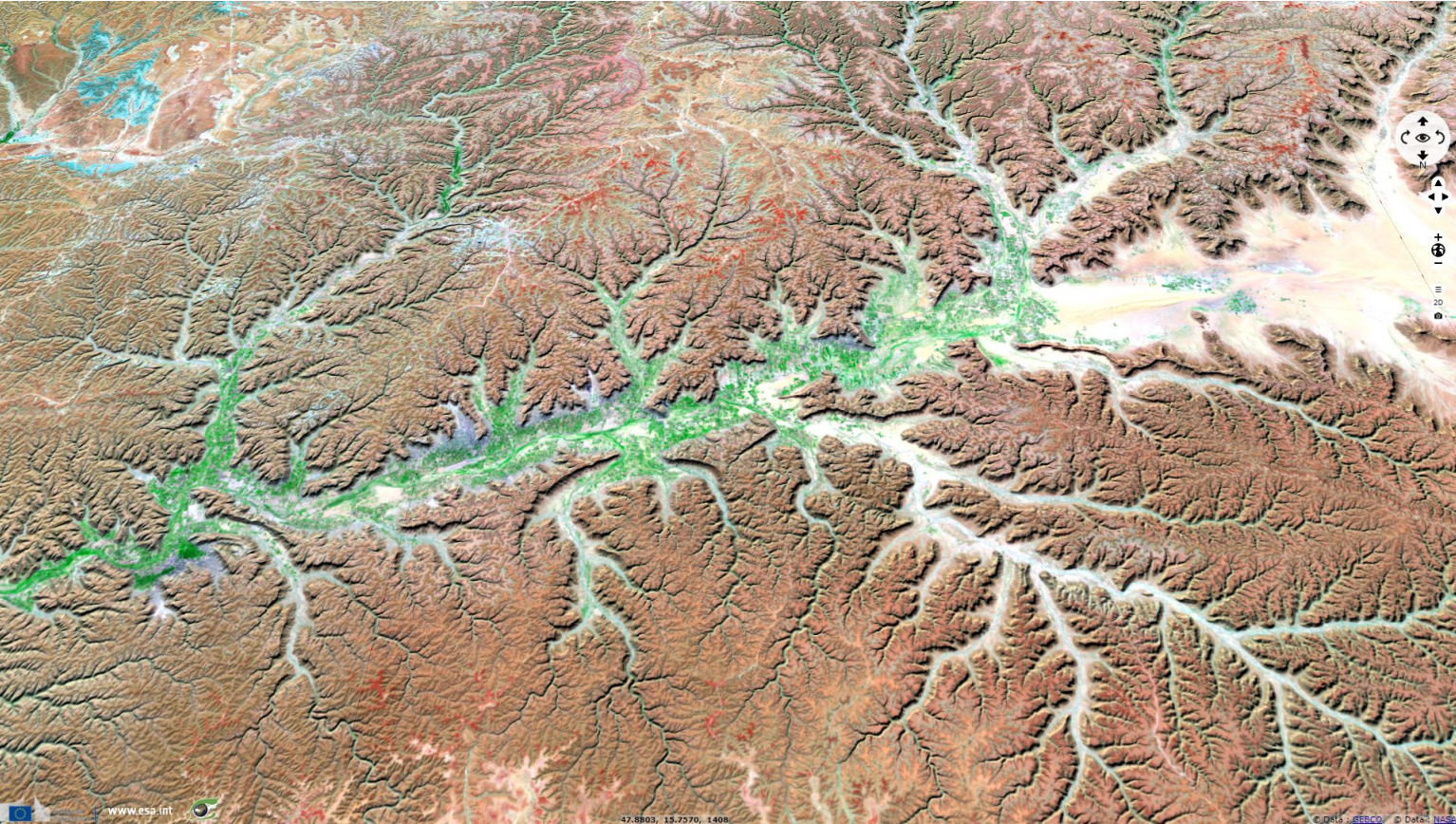
Fig. 5 - S2 - This narrow, arid valley is bounded by the steep escarpment of the al-Jawl broad plateau - 12/8/3 colour composite. 3D view 2D view
