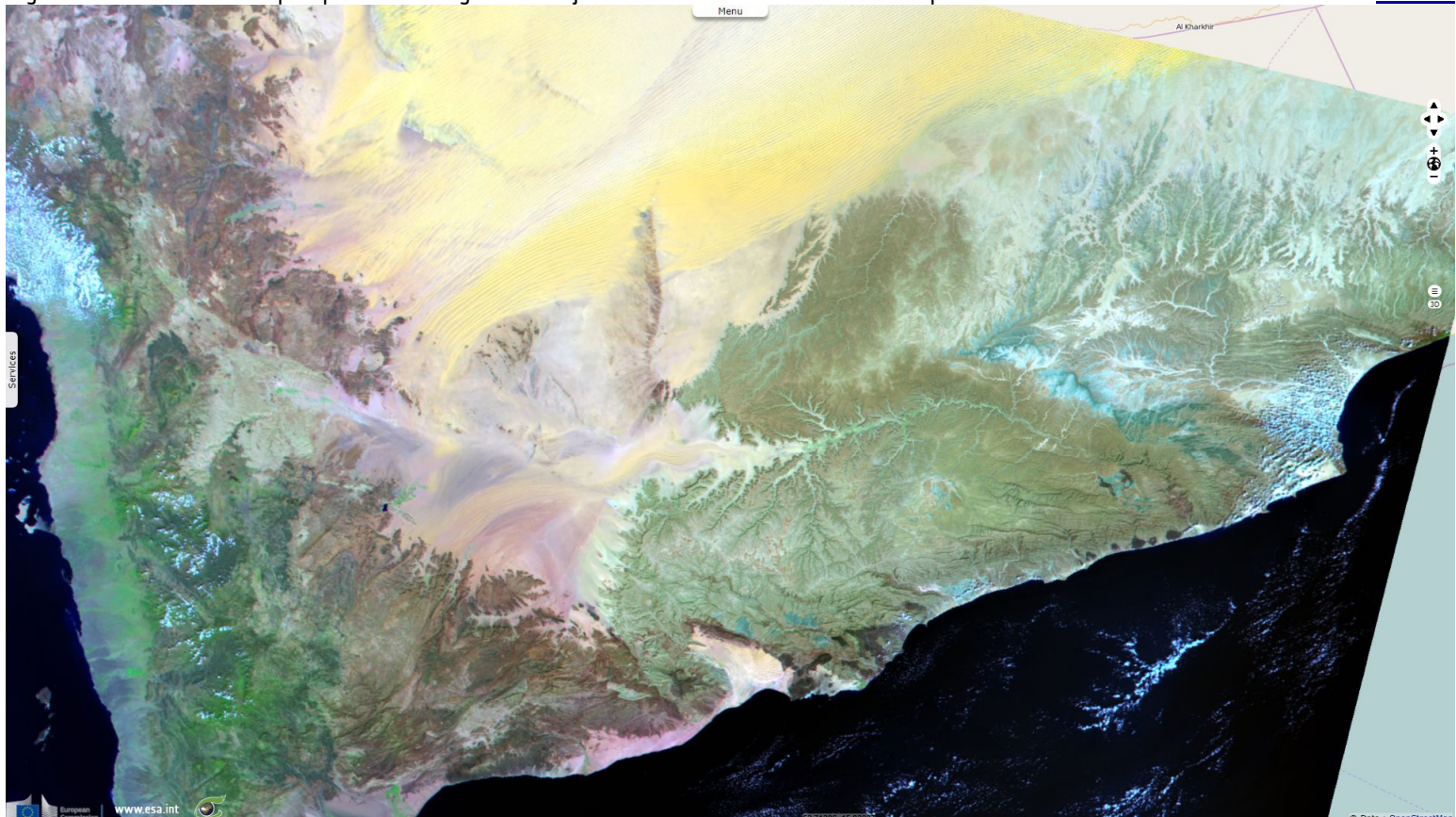
Fig. 2 - SLSTR - Part of the precipitations falling in Yemen joins Gulf of Aden - 6-3-1 colour composite.
