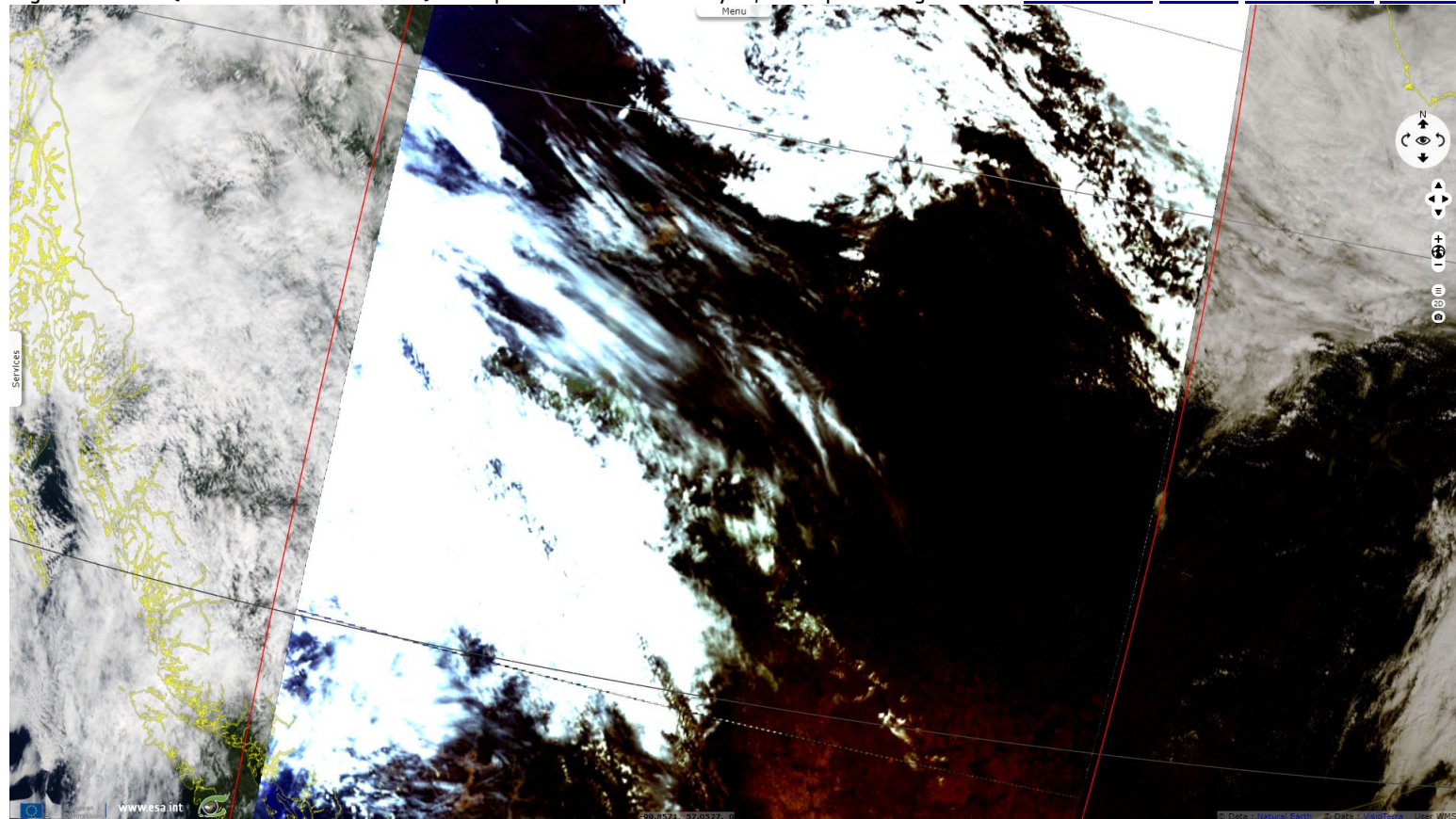
Fig. 4 - S3 SLSTR (21.08.2017 & 25.07.2017) - Comparison with previous cycle, same processing values. 3D animation 3D view 2D animation 2D view
