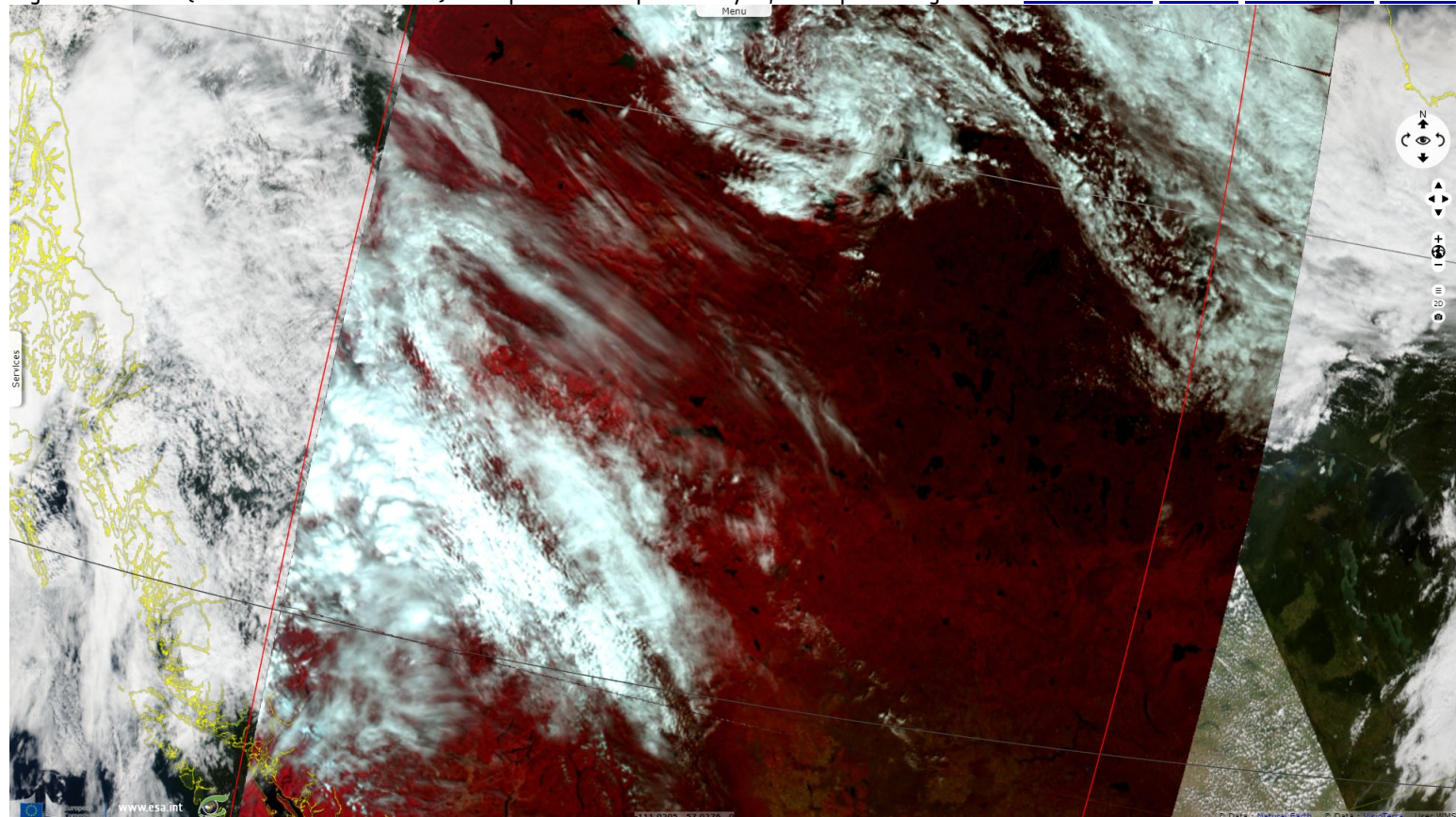
Fig. 4 - S3 SLSTR (21.08.2017 & 25.07.2017) - Comparison with previous cycle, same processing values. 3D animation 3D view 2D animation 2D view
