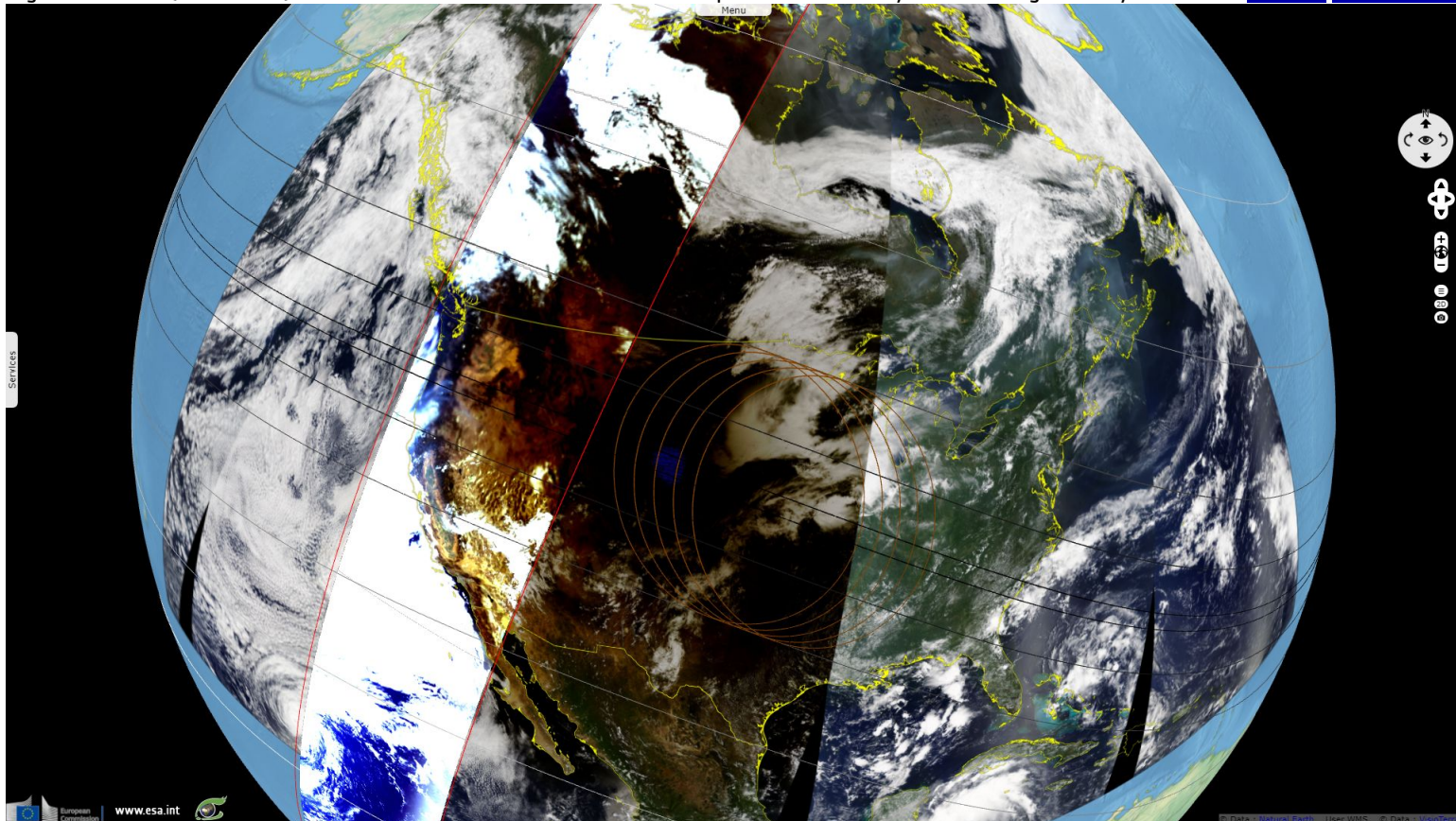
Fig. 2 - S3 SLSTR (21.08.2017) - 3-2-1 colour composite - SLSTR swath over captured VIIRS daily mosaic background layer.
