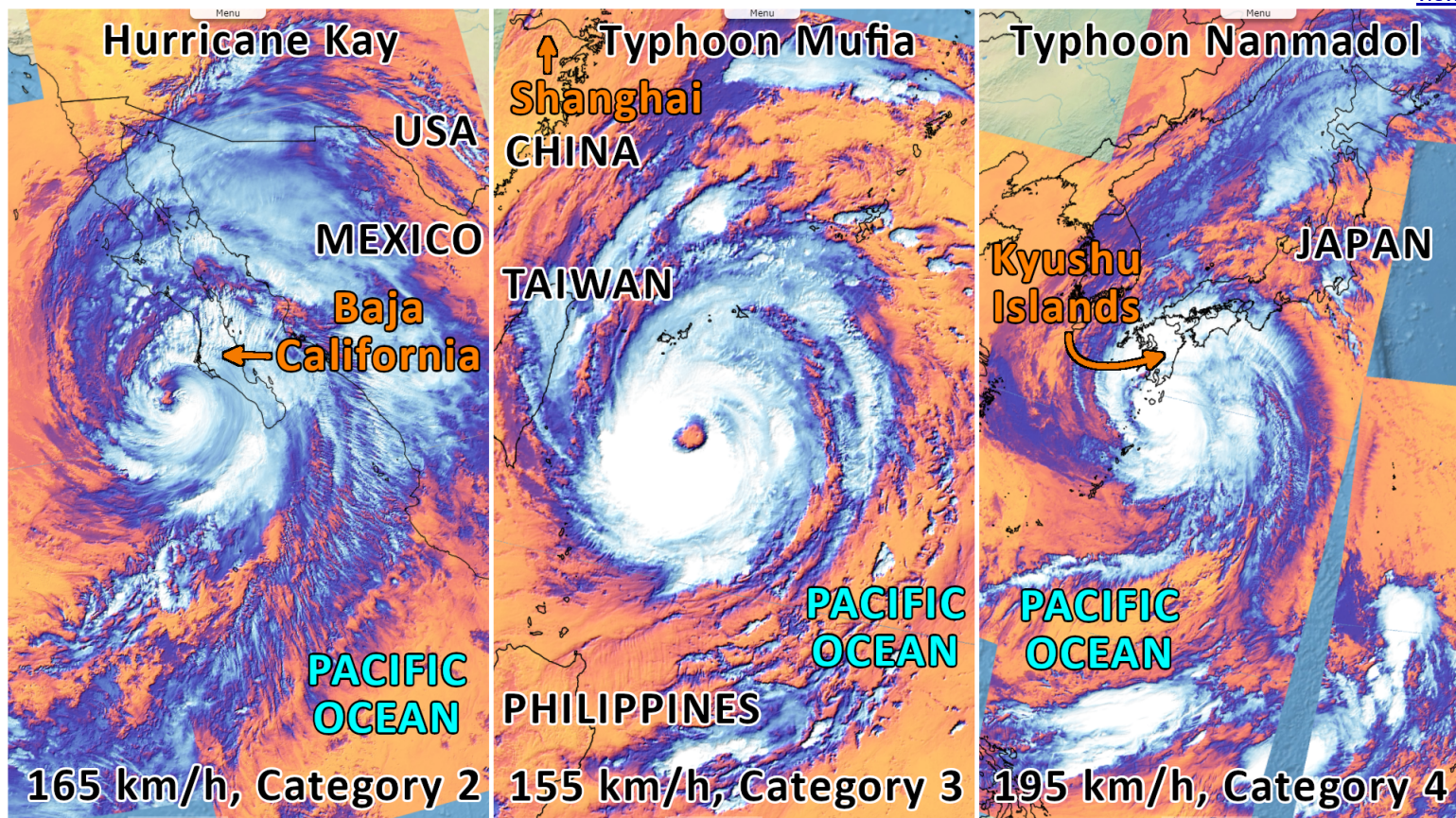
Fig. 2 - S3 SLSTR (08.09.2022; 11.09.2022; 18.09.2022) - Hurricane Kay, Typhoon Mufia & Typhoon Nanmadol all made landfall.
