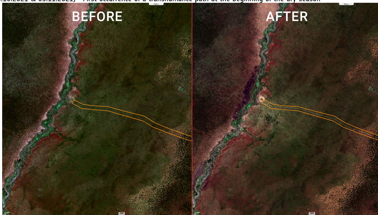
Fig. 2 - S2 (29.10.2021 & 03.11.2021) - First occurrence of a transhumance path at the beginning of the dry season 2D view
