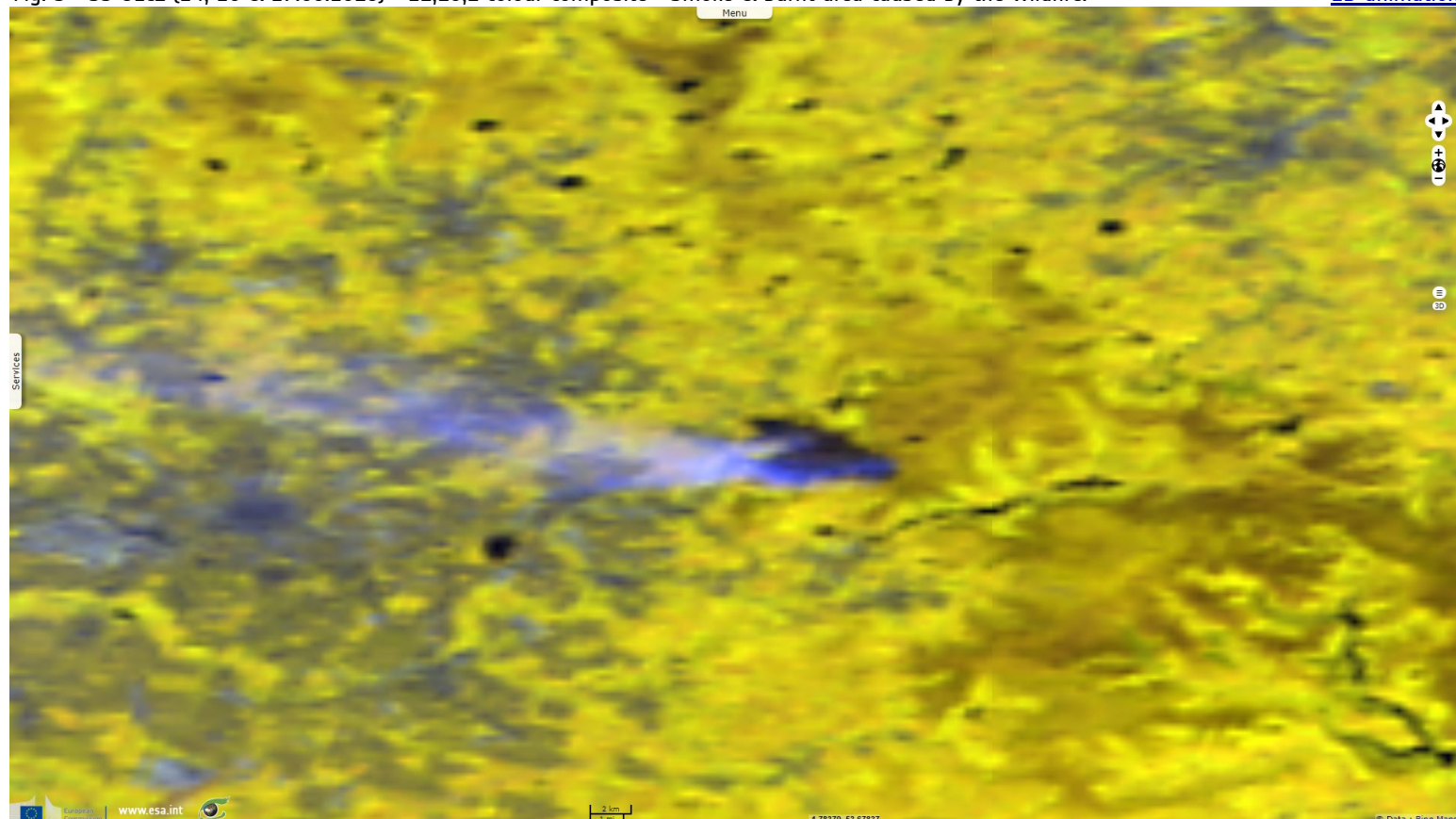
Fig. 4 - S3 SLSTR (24, 25, 26, 27 & 28.06.2018) - S6,S5,S2 colour composite - Fire front & burnt area caused by the wildfire.
