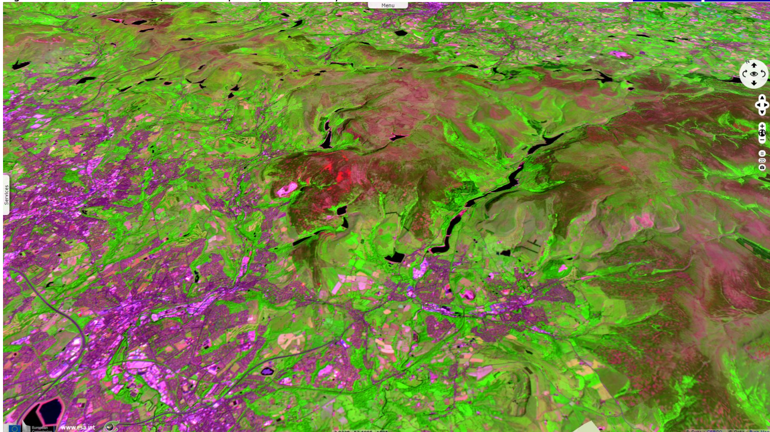
Fig. 2 - S2 (26.06.2018) - 12,11,2 colour composite, relief x3 - The wildfire broke out in the heath landscape.
