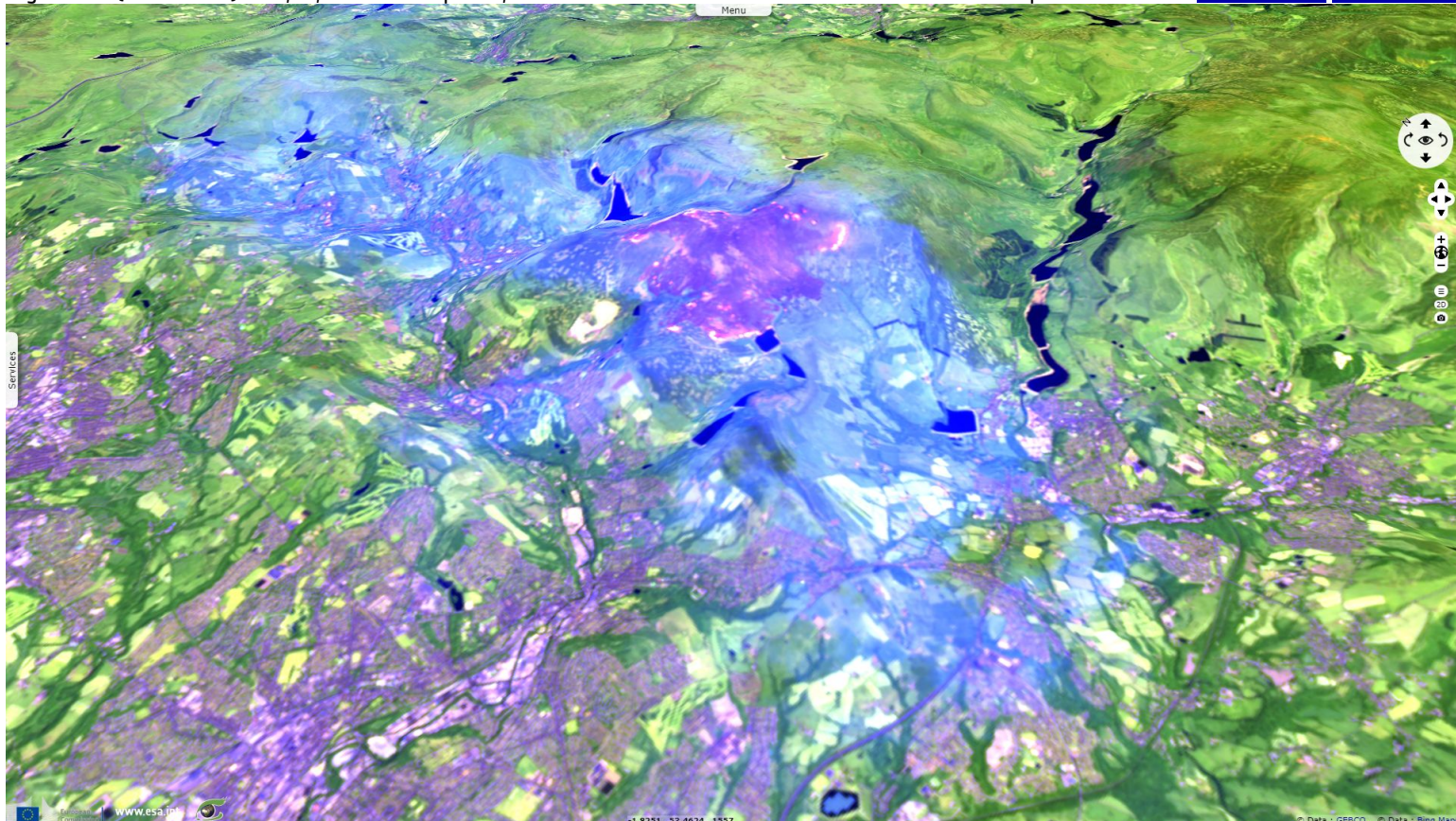
Fig. 2 - S2 (26.06.2018) - 12,11,2 colour composite, relief x3 - The wildfire broke out in the heath landscape.
