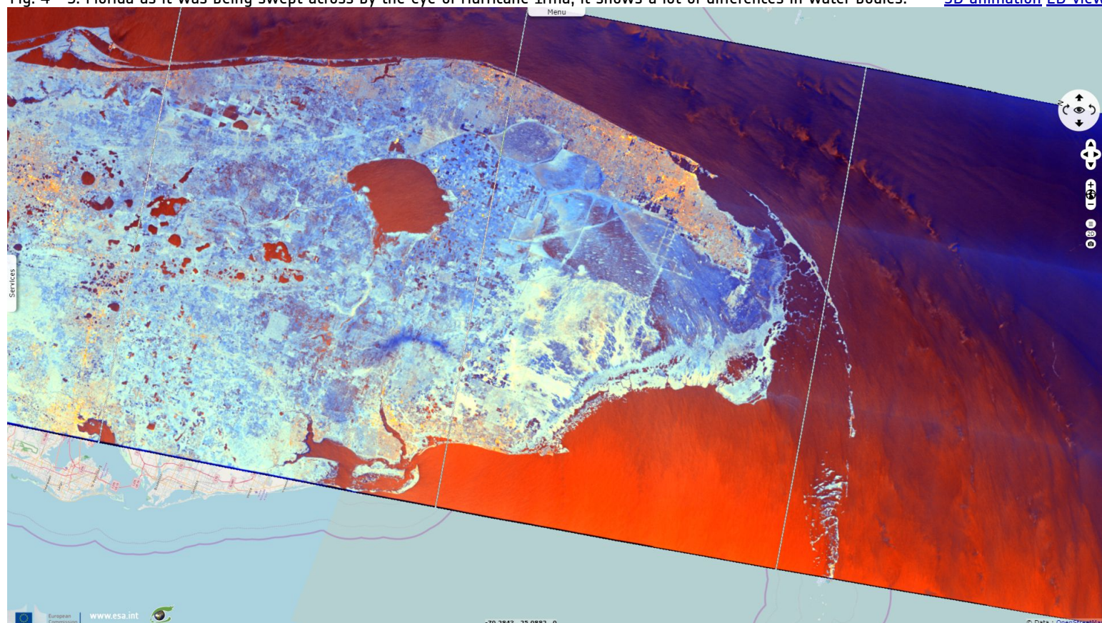
Fig. 4 - S. Florida as it was being swept across by the eye of Hurricane Irma, it shows a lot of differences in water bodies.
