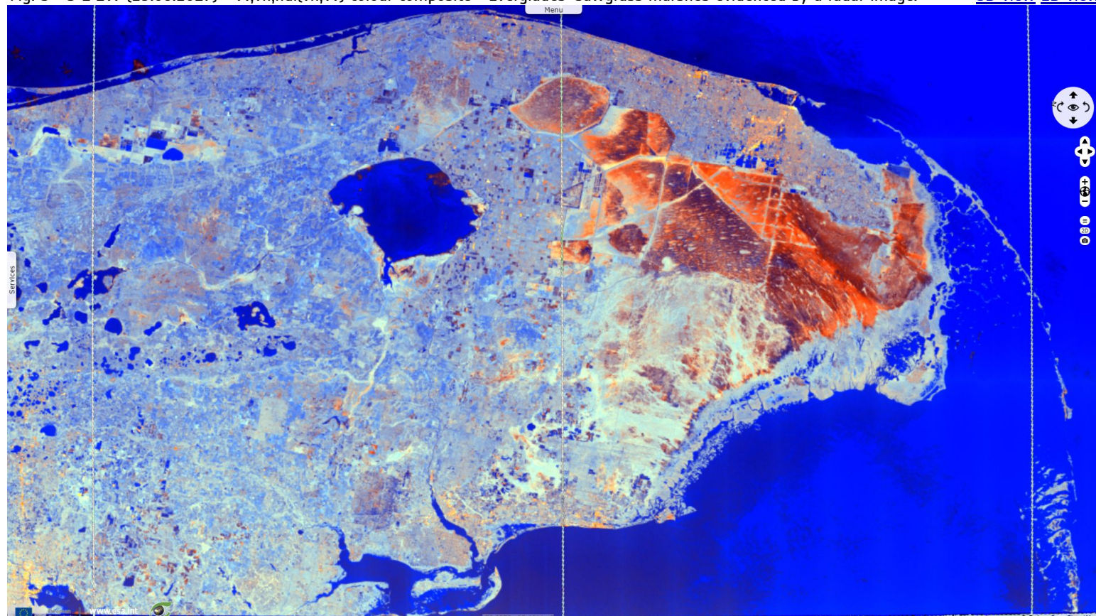
Fig. 4 - S. Florida as it was being swept across by the eye of Hurricane Irma, it shows a lot of differences in water bodies.
