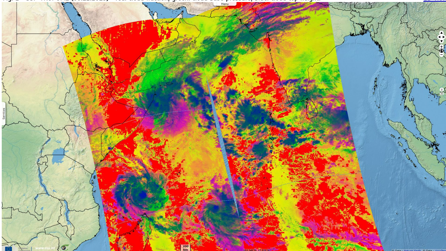
Fig. 2 - S5P TROPOMI (06.12.2019) - red: cloud fraction, green: cloud base pressure, blue: cloud top height.
