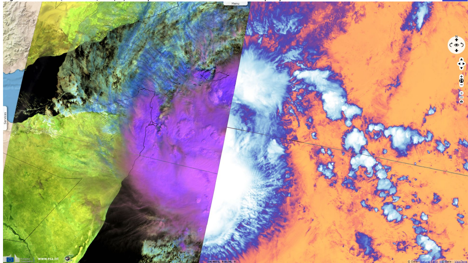
Fig. 5 - S3 SLSTR (06.12.2019) - S6,S5,S2 composite / Thermal band with colour map - Cyclonic storm Pawan caused flash floods in Somalia. 2D view
