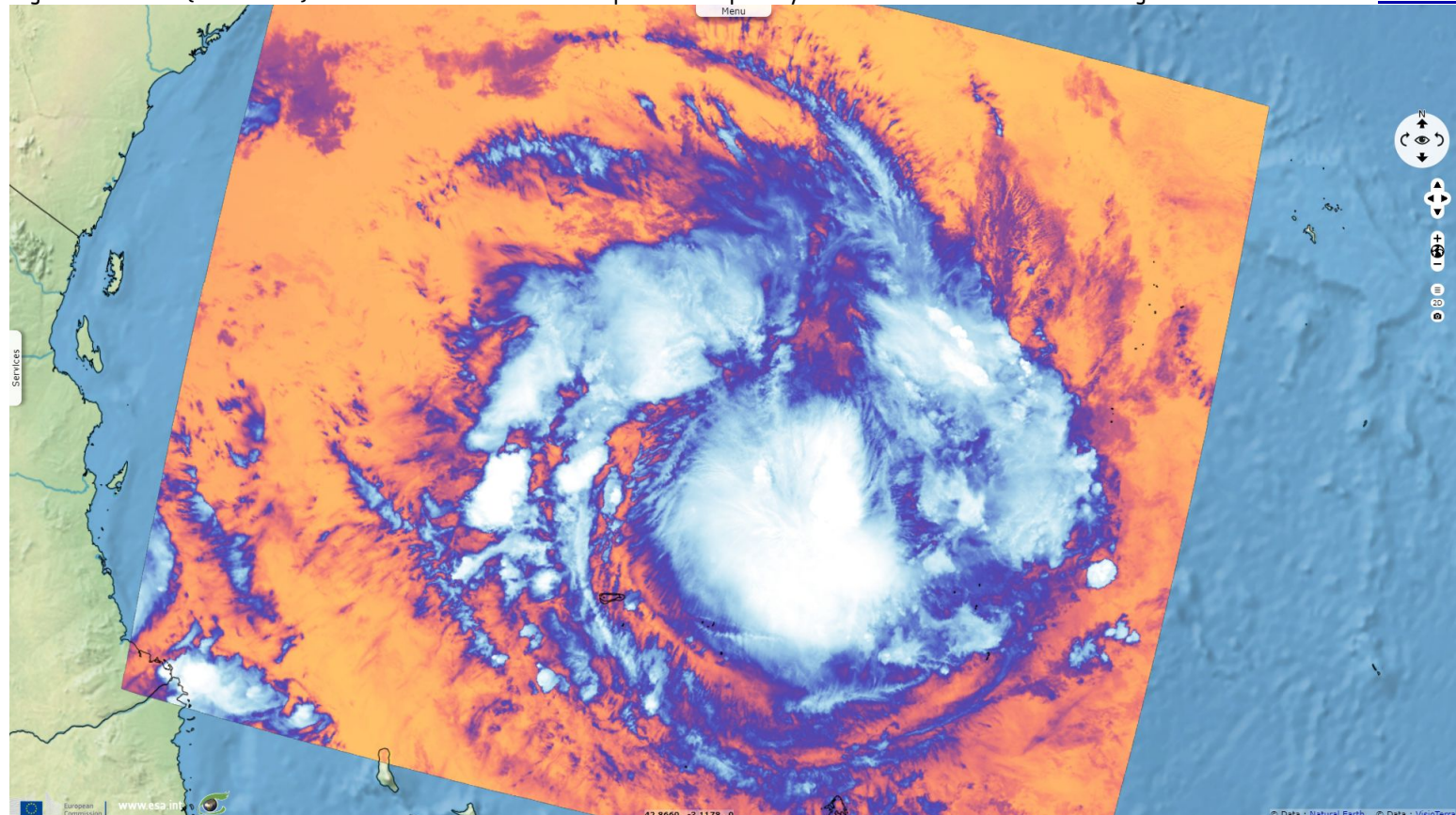
Fig. 4 - S3 SLSTR (06.12.2019) - Thermal band with colour map - Cat.3 tropical Cyclone Belna made landfall on Madagascar on 09.12.2019.
