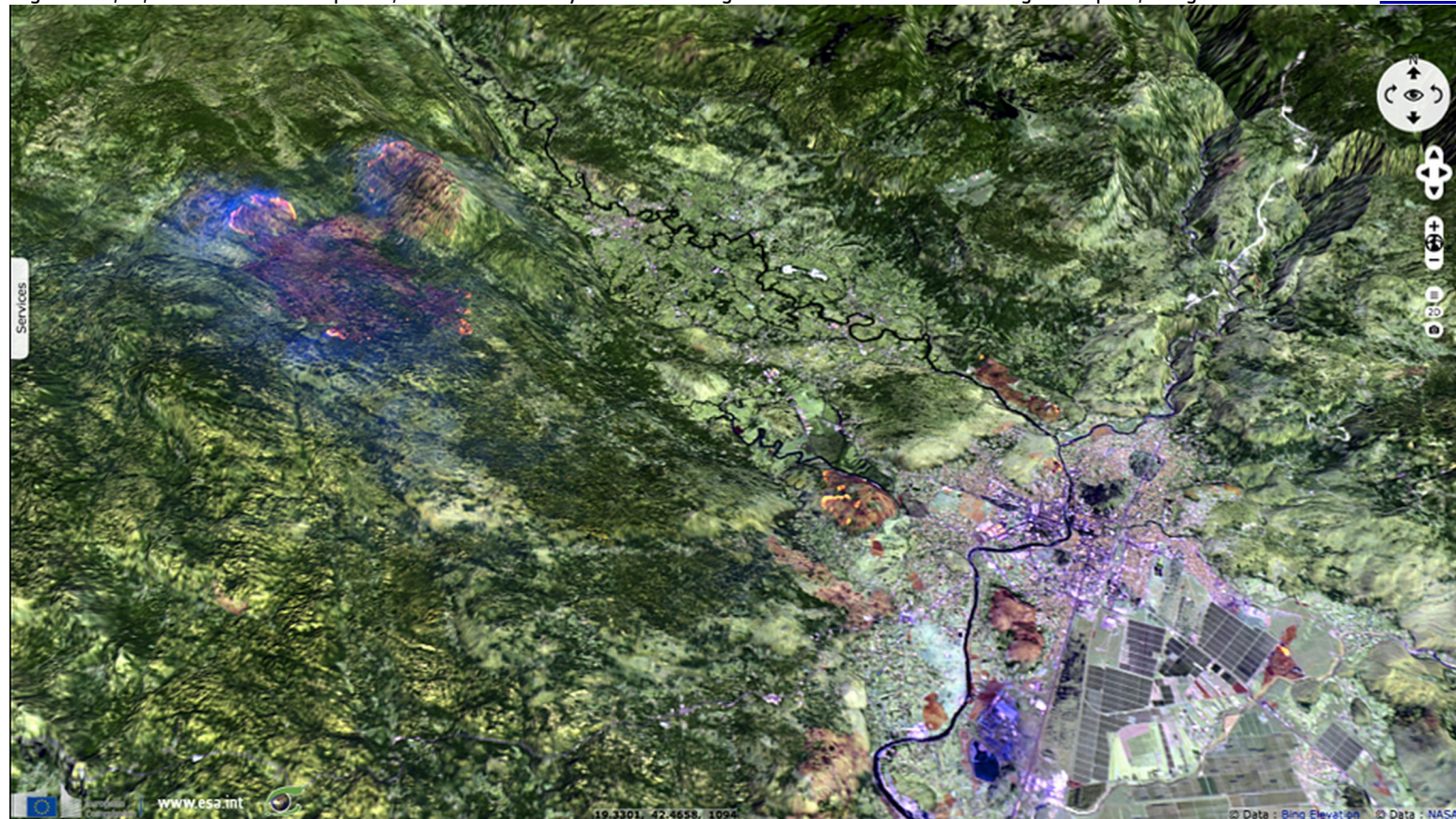
Fig. 4 - 8,4,3 Vegetation colour composite - Piva river surrounded by mountains, forming a canyon.
