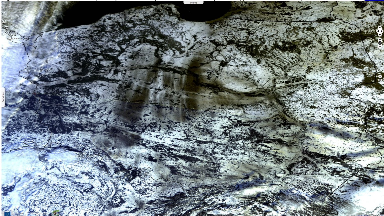
Fig. 2 - On this image (11.01.2017), SLSTR better discriminates snow from clouds, and grassland from forests - 6-3-2 colour composite.
