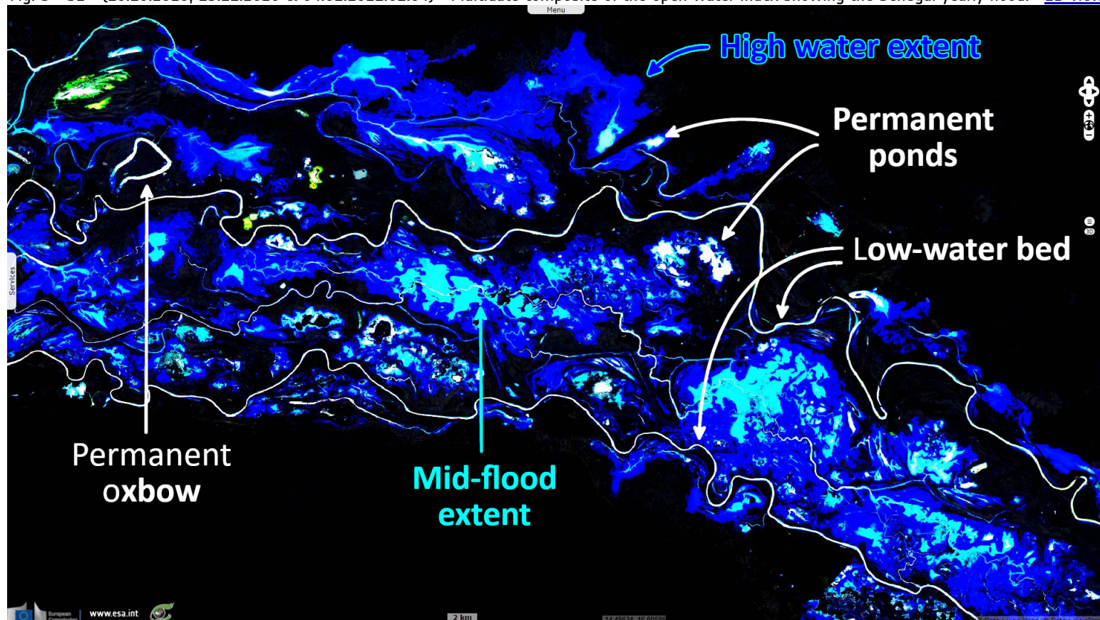
Fig. 6 - S2 (17.03.2022) - The meanders of Sénégal river evolve along time, leaving meander scars of the past path of the river. 2D view
