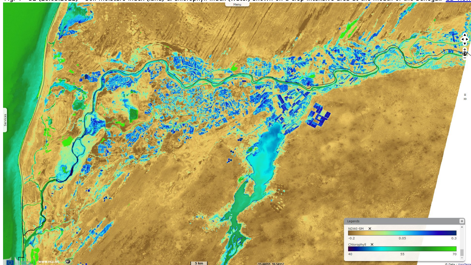
Fig. 4 - S2 (18.03.2022) - Soil moisture index (land) & Chlorophyll index (water) shown on a crop intensive area at the mouth of the Sénégal. 2D view
