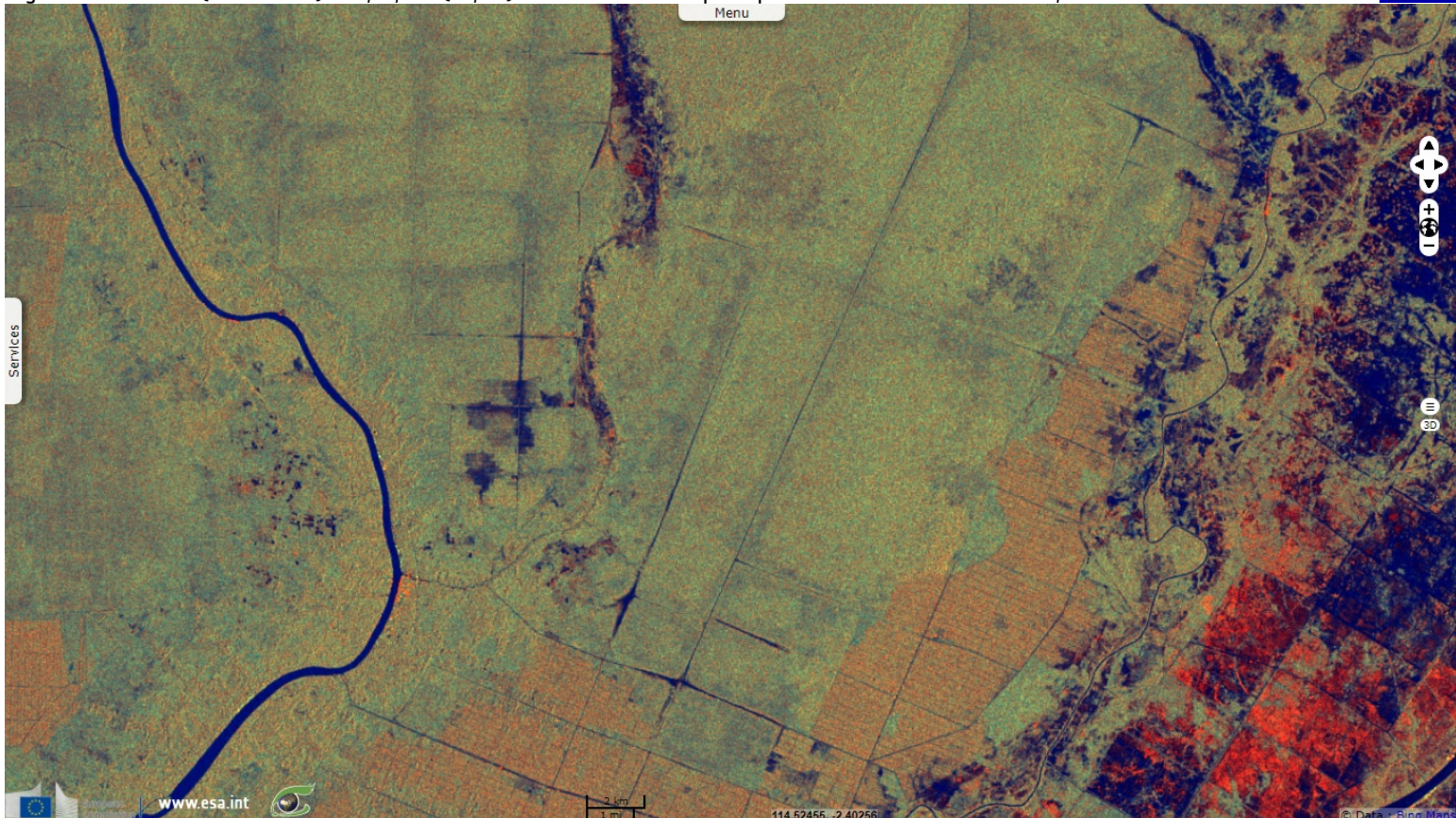
Fig. 2 - Sentinel 1A (07.12.2017) - vv,vh, ndi (vh, vv) orthorectified - Oil palm plantations in southern Borneo, Indonesia.
