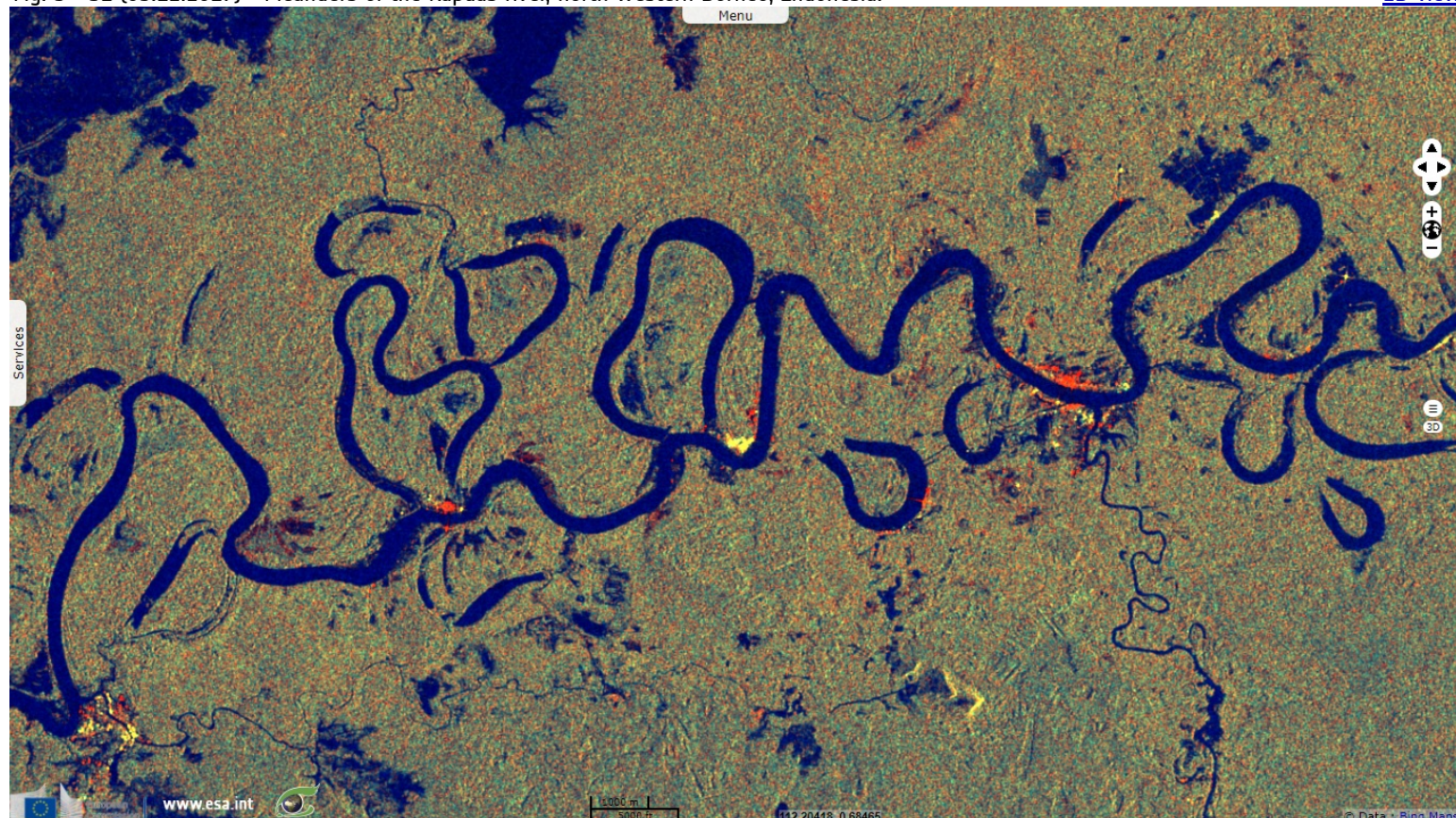
Fig. 4 - S2 (20.07.2017) - 8,4,3 Vegetation colour composite - Mangroves and crops, north eastern Borneo, Indonesia.
