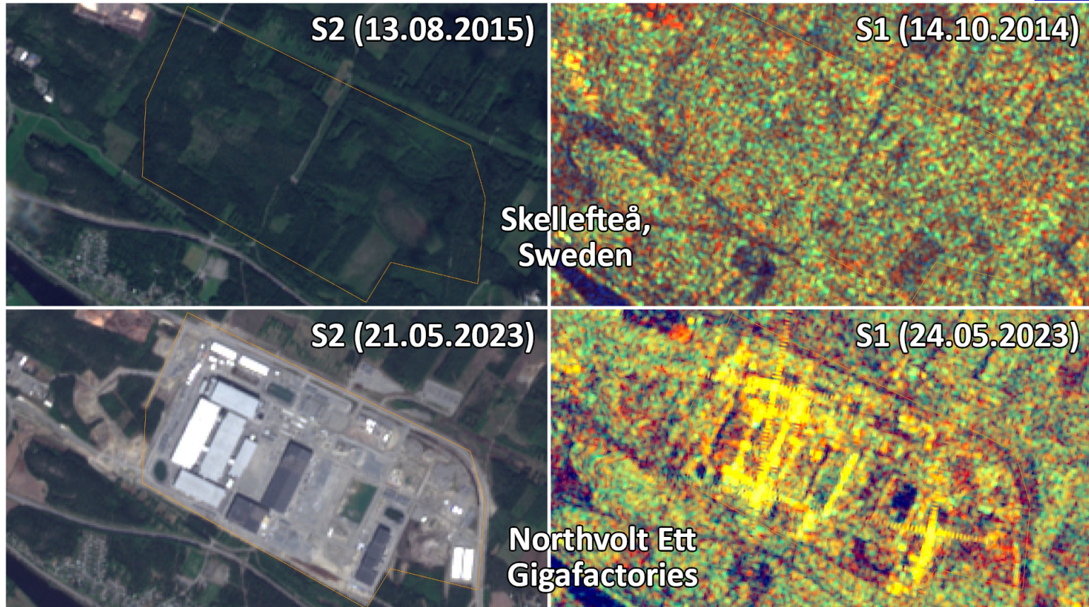
Fig. 1 - S2 (13.08.2015; 21.05.2023); S1 (14.10.2014; 24.05.2023) - Northvolt Ett battery gigafactory in Skellefteå, Sweden. 3D view 3D view 3D view 3D view
