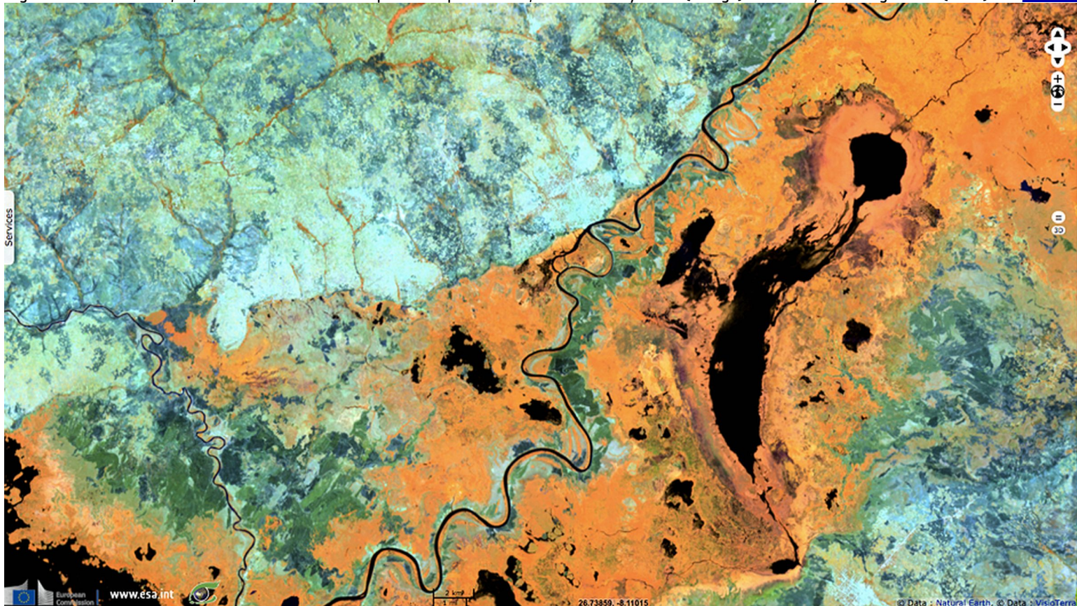
Fig. 2 - Sentinel 2A - 8,11,4 Land/Water colour composite - Upemba lake, in the marshy basin (orange) formed by the Congo River (black).
