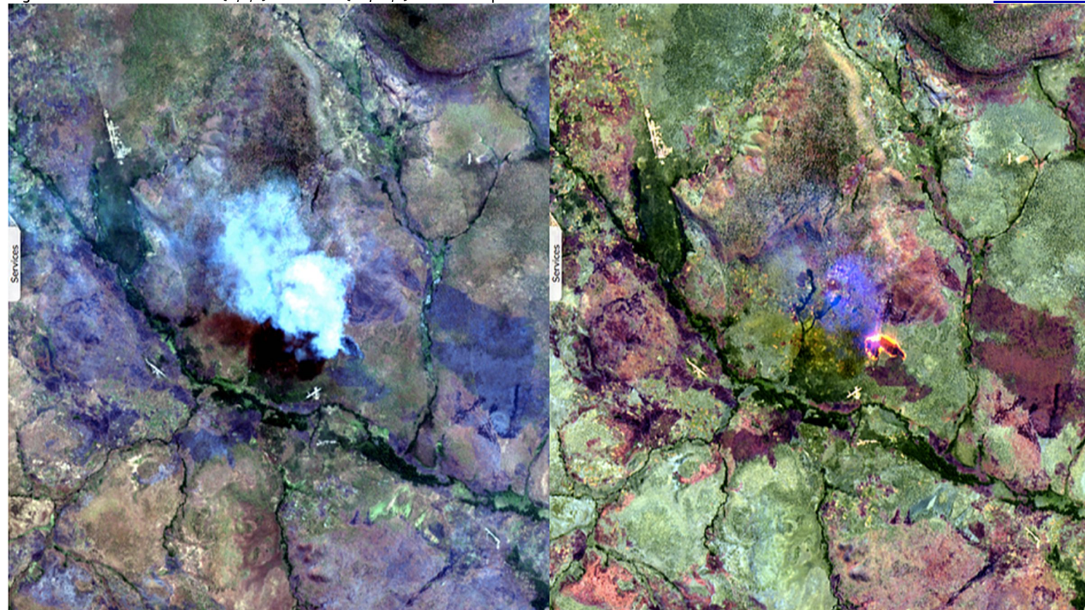
Fig. 4 - Sentinel 2A - 4,3,2 Natural colour composite - Kabalo city along the Congo river.
