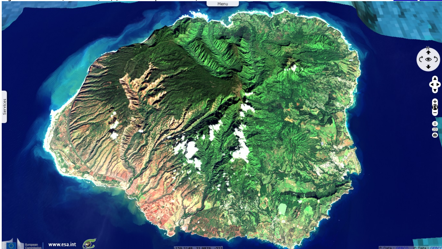
Fig. 2 - Sentinel 2A (2018-01-14) - 4,3,2 colour composite - Kauai, the oldest of the main Hawaiian Islands.
