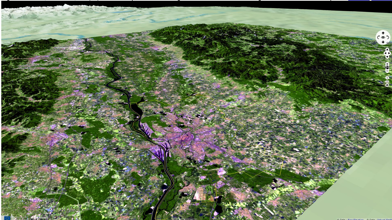
Fig. 2 - S2 MSI (19.06.2017) - 12,11,4 colour composite - Dense vegetation concentrates on the higher hillsides of Rhine valley. 3D view 2D view
