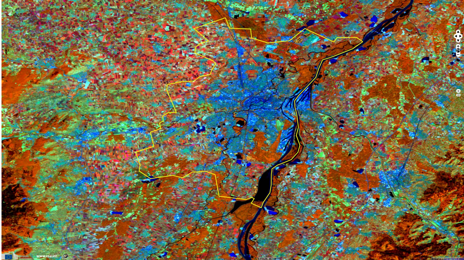
Fig. 1 - S2 MSI (19.06.2017) - 8,11,2 colour composite - Strasbourg Eurometropolis, delimited from Kehl in Germany by the Rhine. 2D view 3D view
