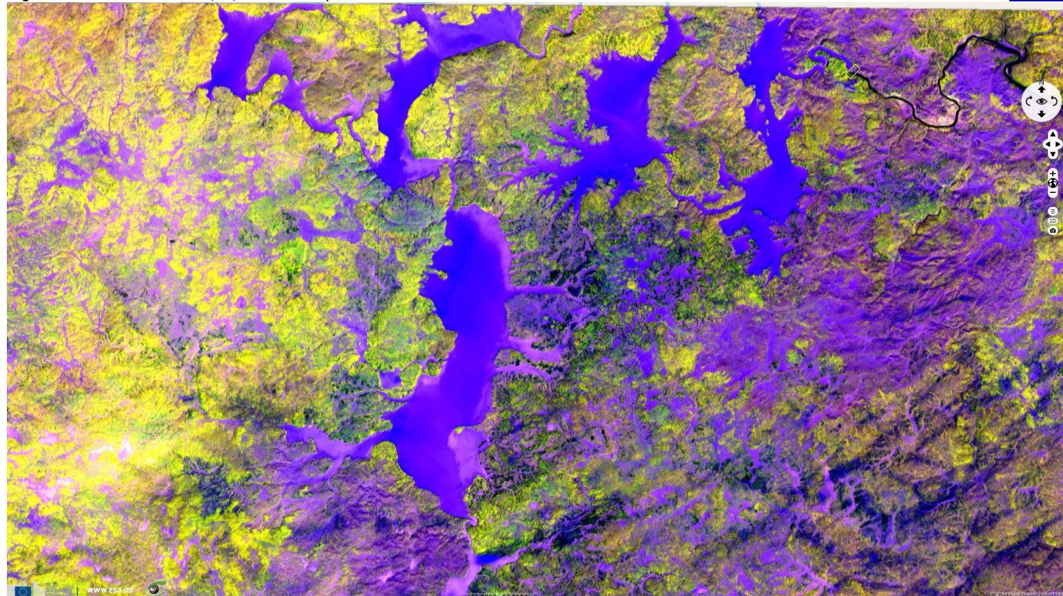
Fig. 4 - 09.04.2018 - vv,vh,ndi(vh,vv) colour composite - S1 shows channels in Chona lake system not visible on S2 acquisitions 2 days after. 3D view
