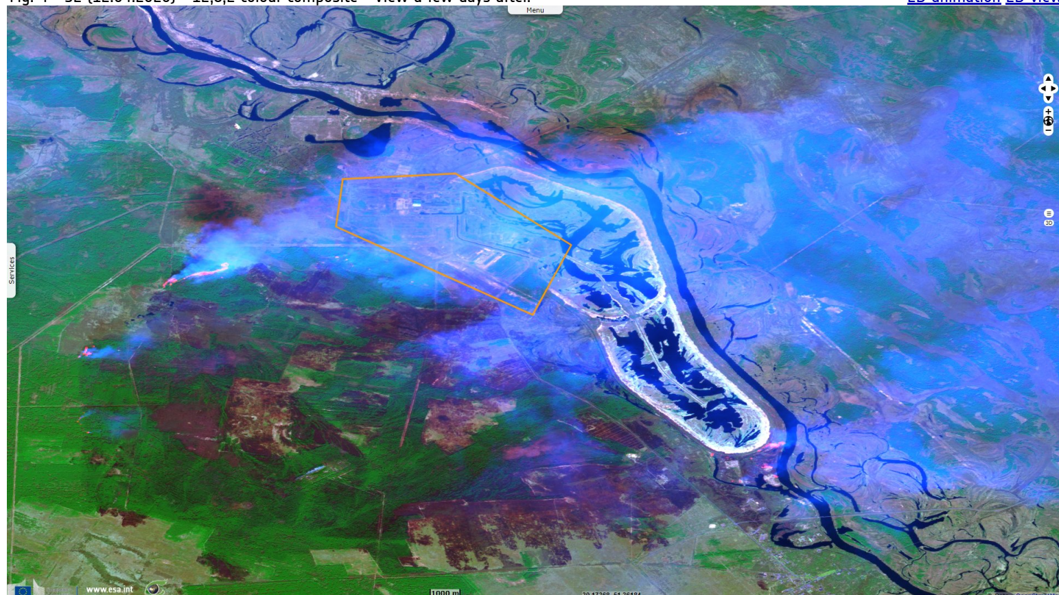
Fig. 4 - S2 (12.04.2020) - 12,8,2 colour composite - View a few days after.
