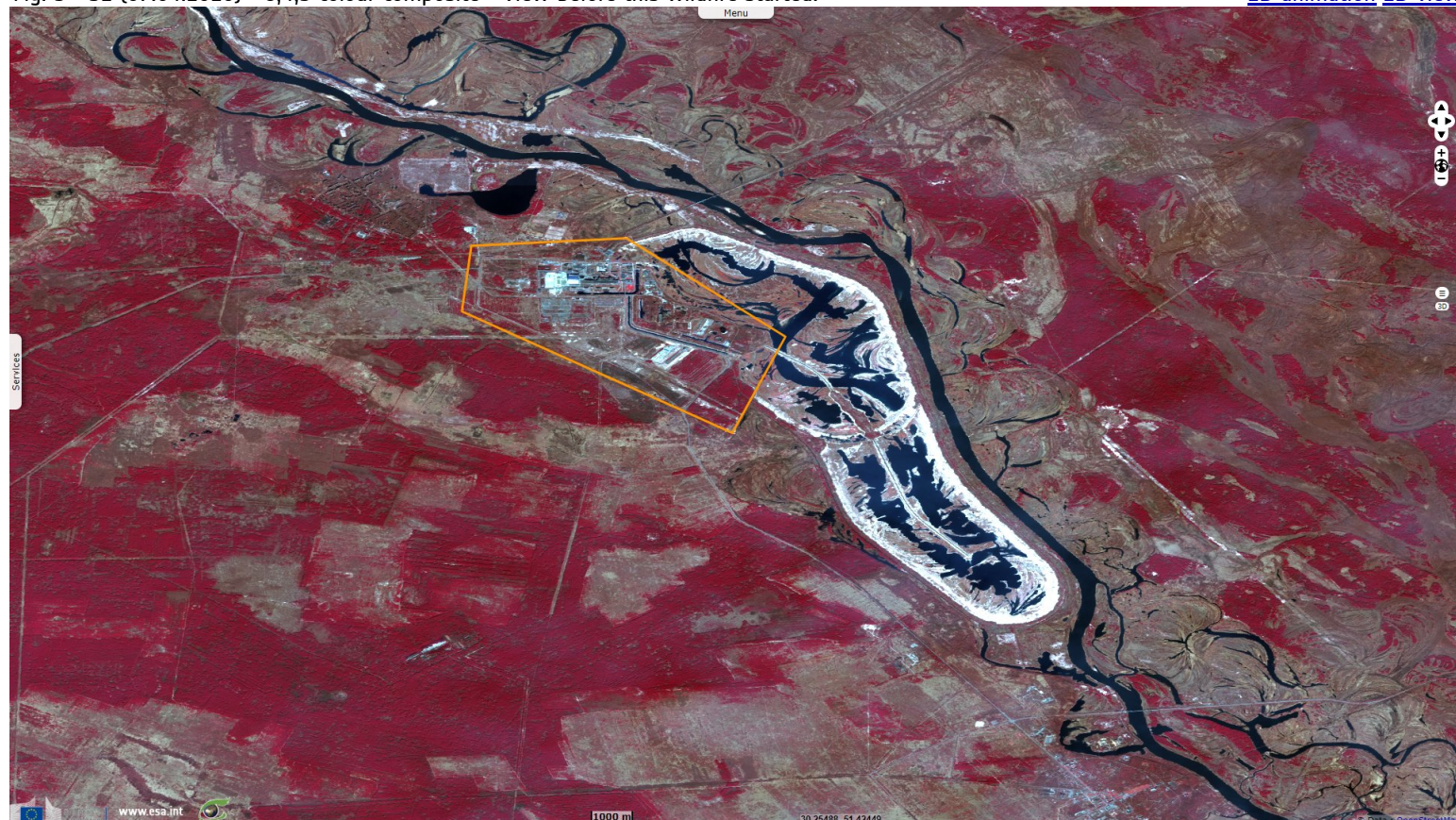
Fig. 4 - S2 (12.04.2020) - 12,8,2 colour composite - View a few days after.
