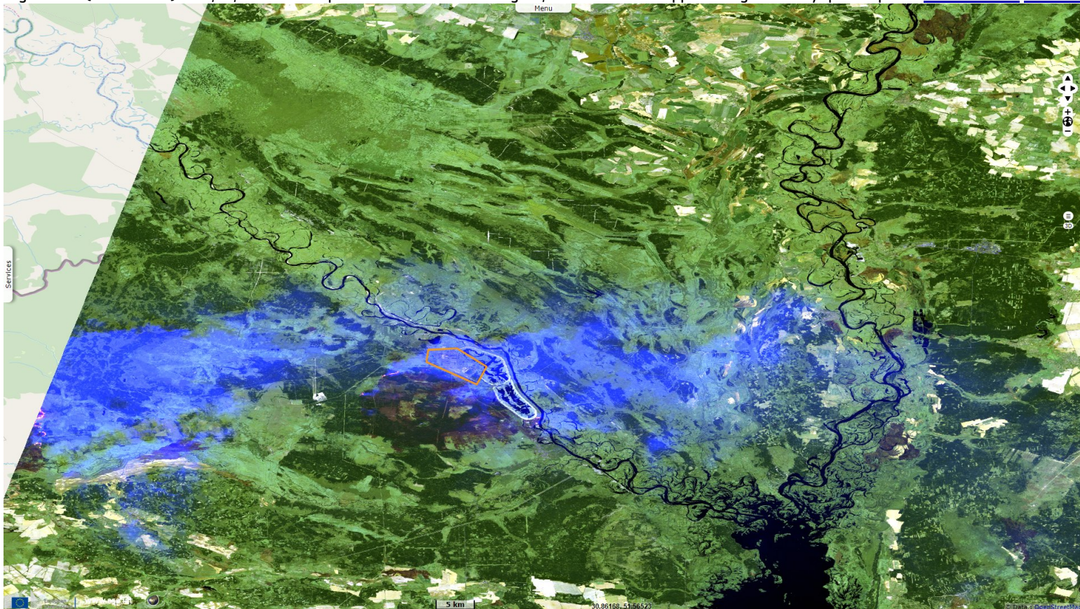
Fig. 2 - S2 (12.04.2020) - 12,11,2 colour composite - While not the largest, one of these is approaching Chernobyl power plant. 2D animation 2D view
