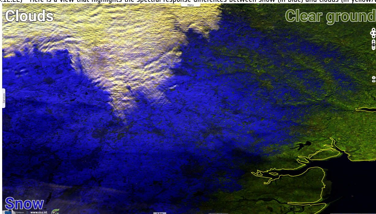
Fig. 2 - S2 (14.12.22) - Here is a view that highlights the spectral response differences between snow (in blue) and clouds (in yellow/white). 2D view
