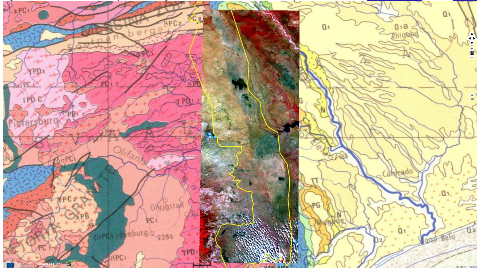
Fig. 4 - S2A MSI - 11-8-2 colour composite - Wayne LOTTER was assassinated August 16, 2017 in Dar es Salaam.
