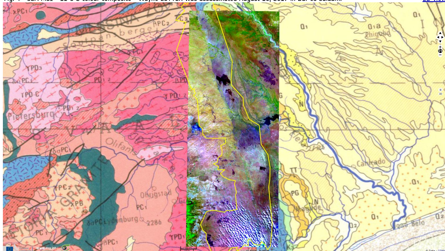
Fig. 4 - S2A MSI - 11-8-2 colour composite - Wayne LOTTER was assassinated August 16, 2017 in Dar es Salaam.
