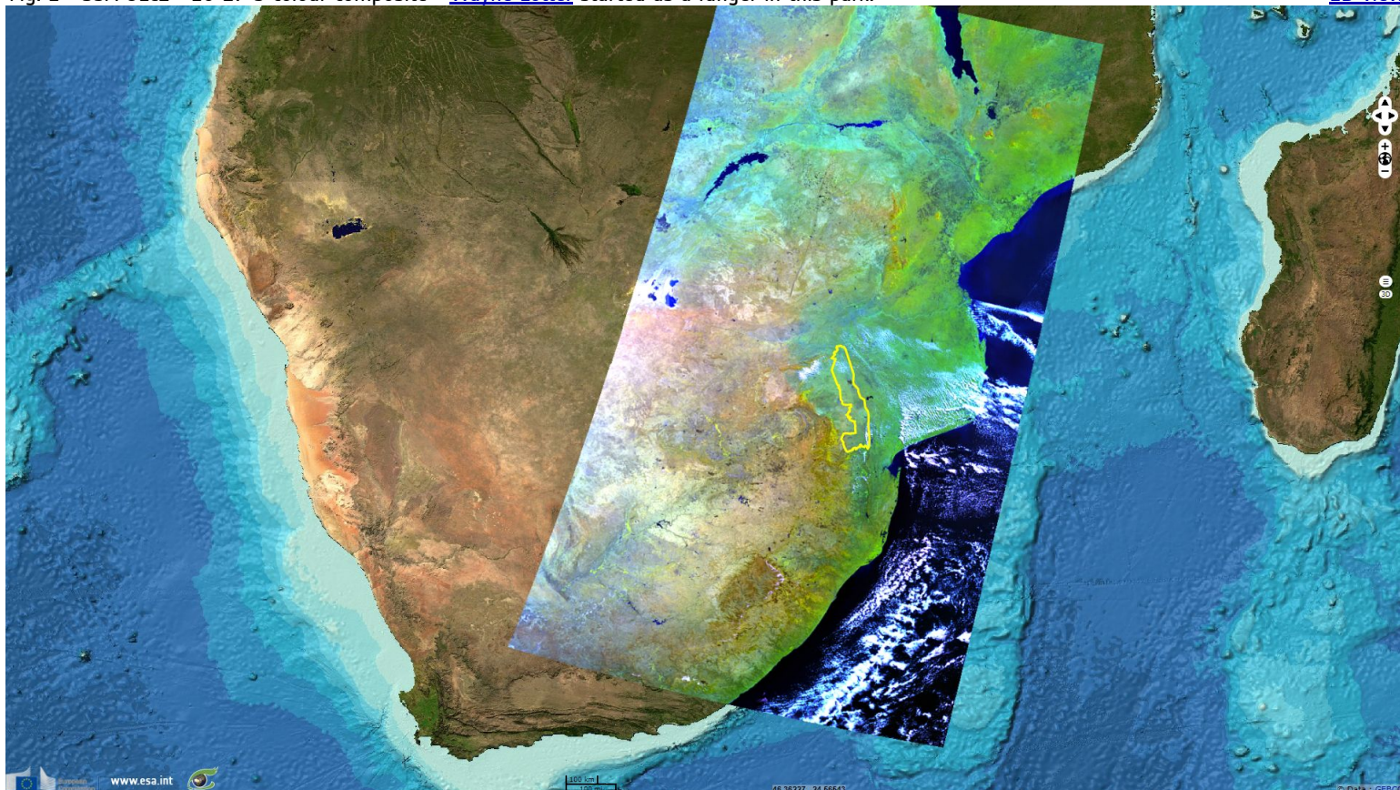
Fig. 2 - S3A OLCI - 20-17-5 colour composite - Wayne Lotter started as a ranger in this park.
