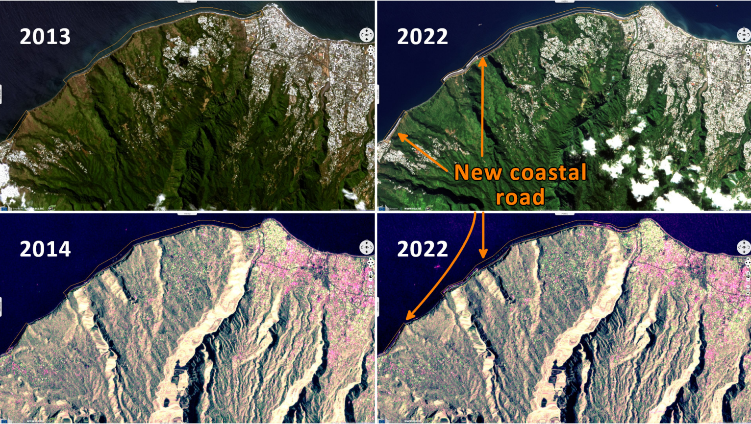
Fig. 2 - L8 (19.09.2013), S2 (26.05.2022), S1 (04->28.10.2014; 30.07->23.08.2022) - This road is very costly due to technical difficulties. 3D view 3D view 3D view 3D view
