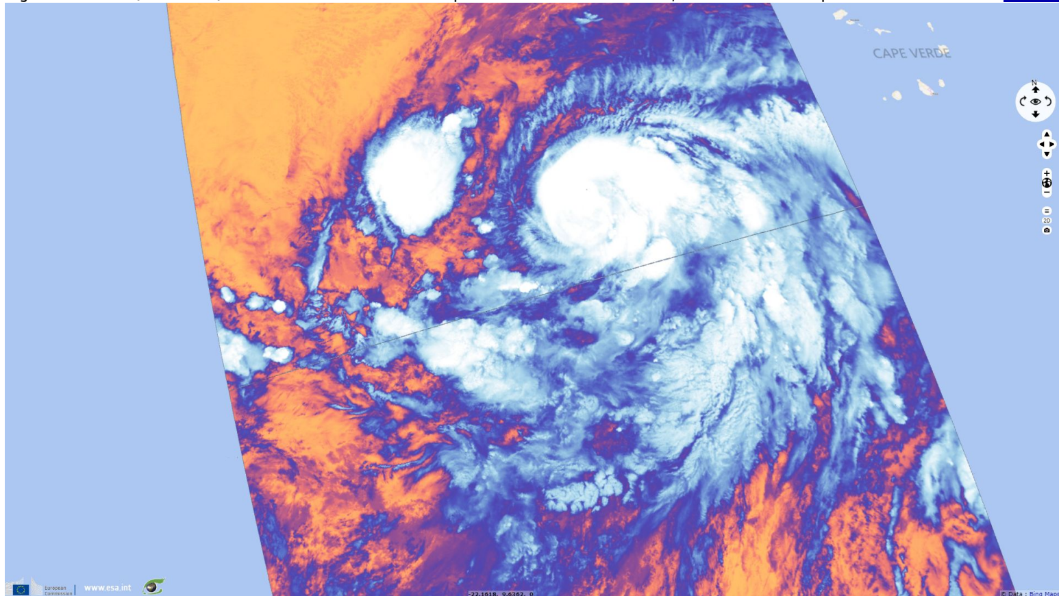
Fig. 2 - S3 SLSTR (26.09.2019) S8 thermal band with colour map.
