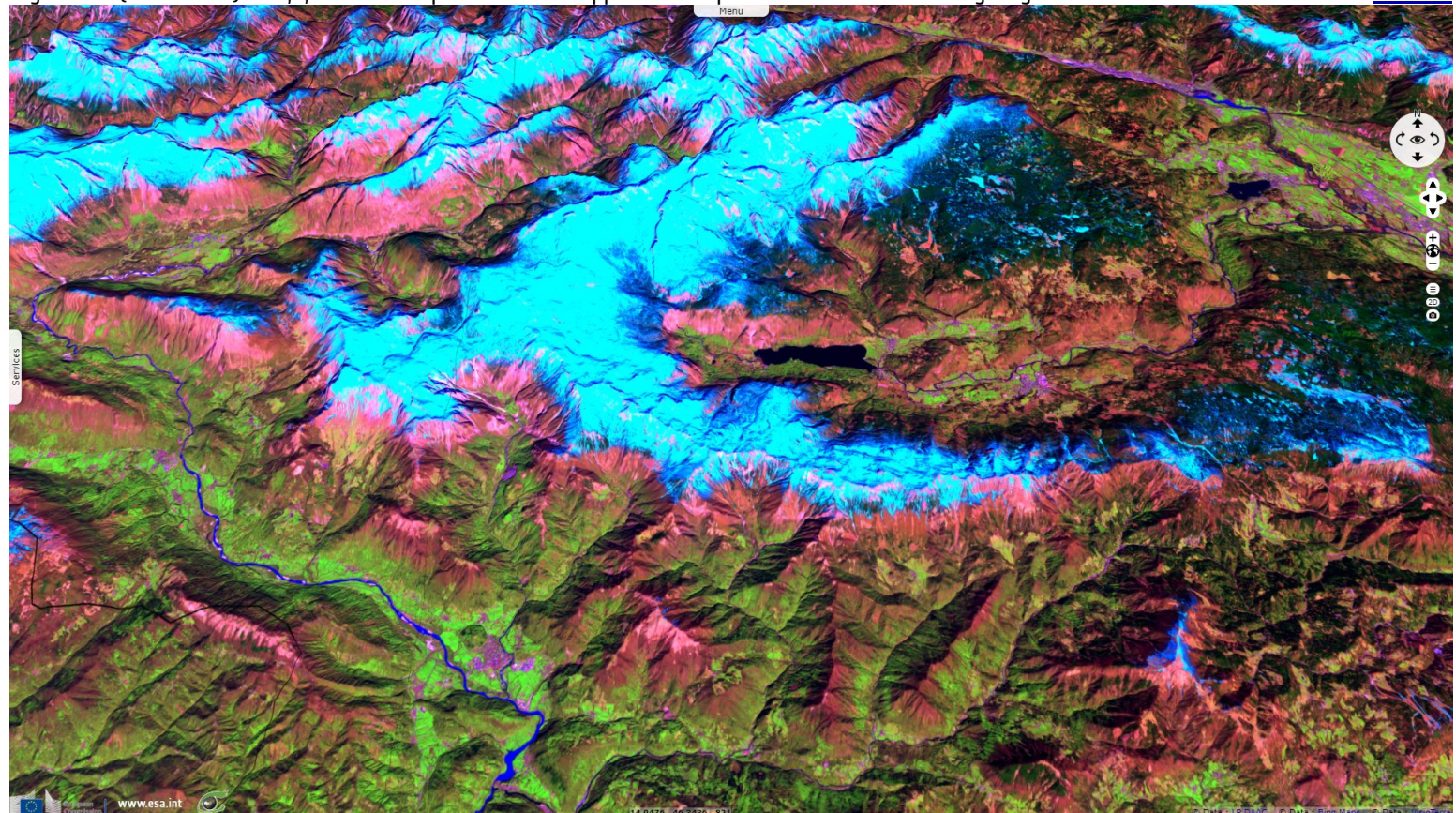
Fig. 4 - S2 (21.04.2019) - 11,8,2 colour composite - Snow capped landscape two months earlier - Triglav glacier lost its status in 2019. 3D view
