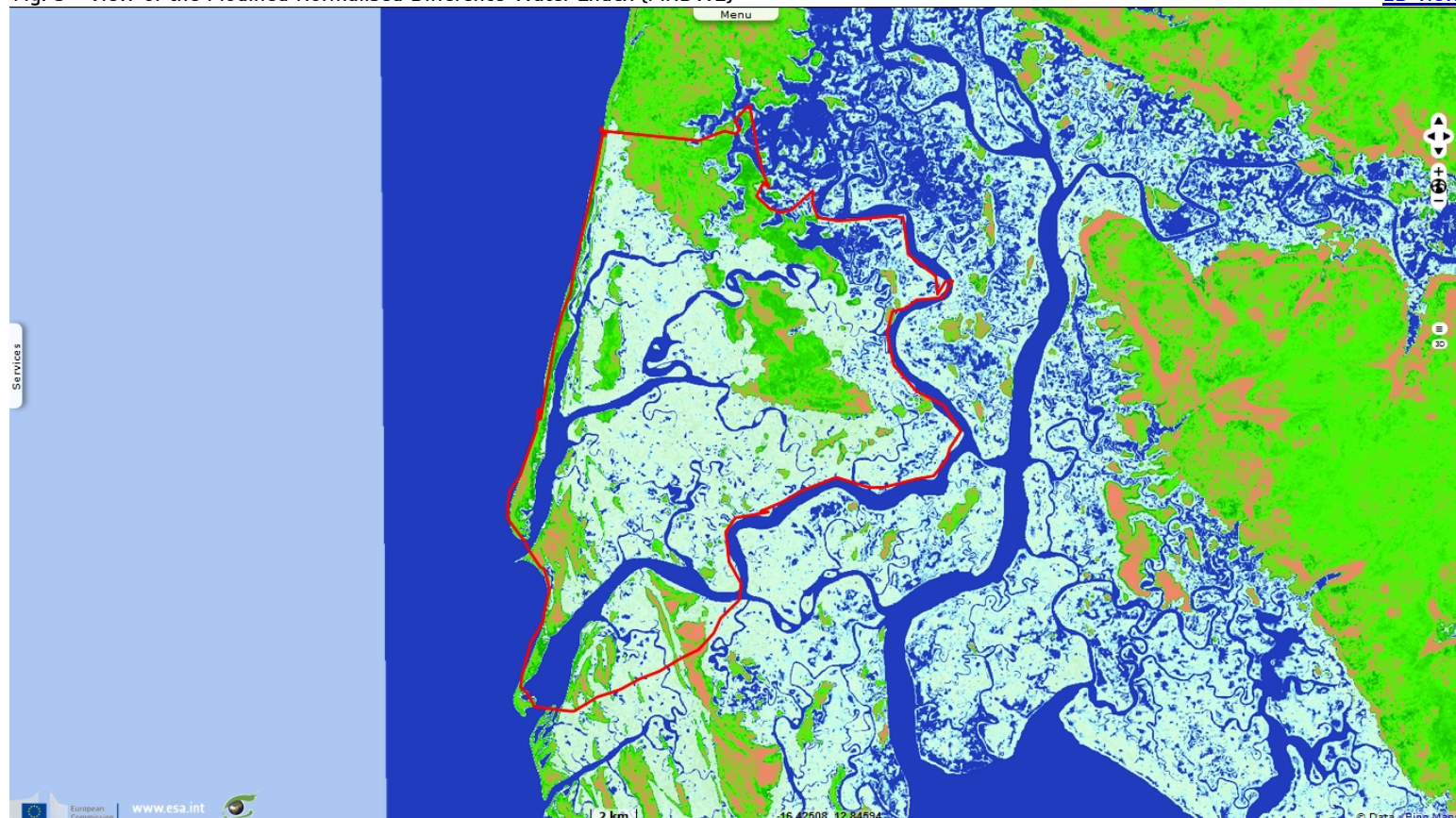
Fig. 6 - Land use map extracted from vegetation and water indices
