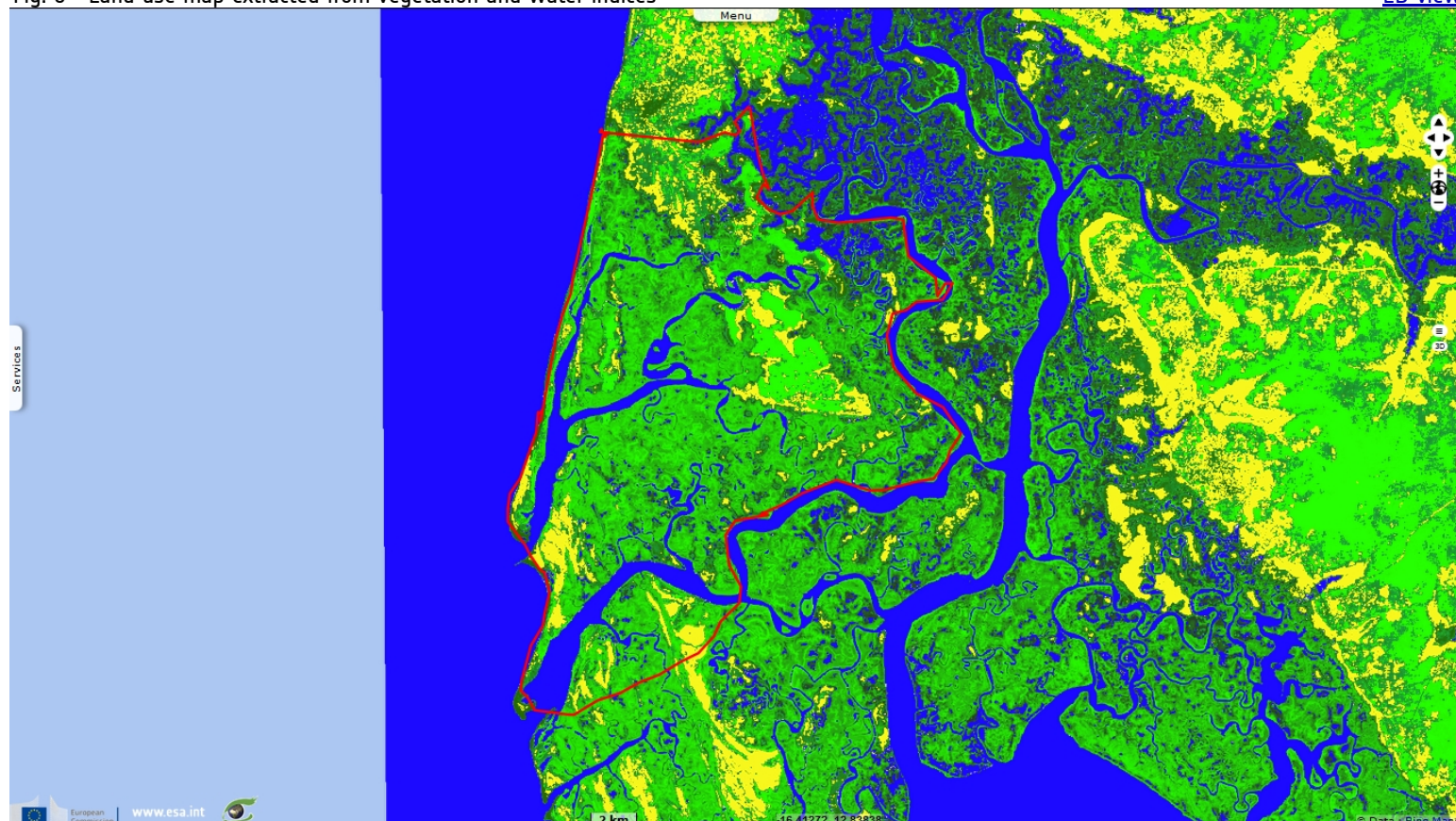
Fig. 6 - Land use map extracted from vegetation and water indices
