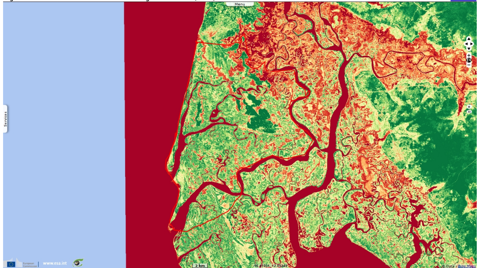
Fig. 4 - View of the Normalised Difference Water Index for Soil Moisture (NDWI-SM)
