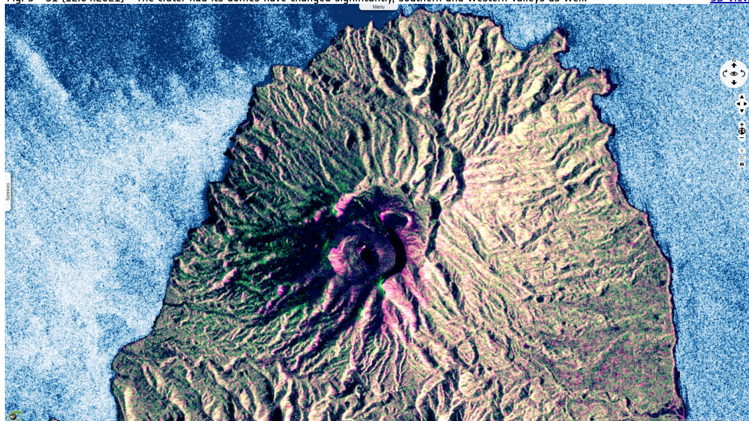
Fig. 5 - S1 (12.04.2021) - The crater had its domes have changed significantly, southern and western valleys as well.
