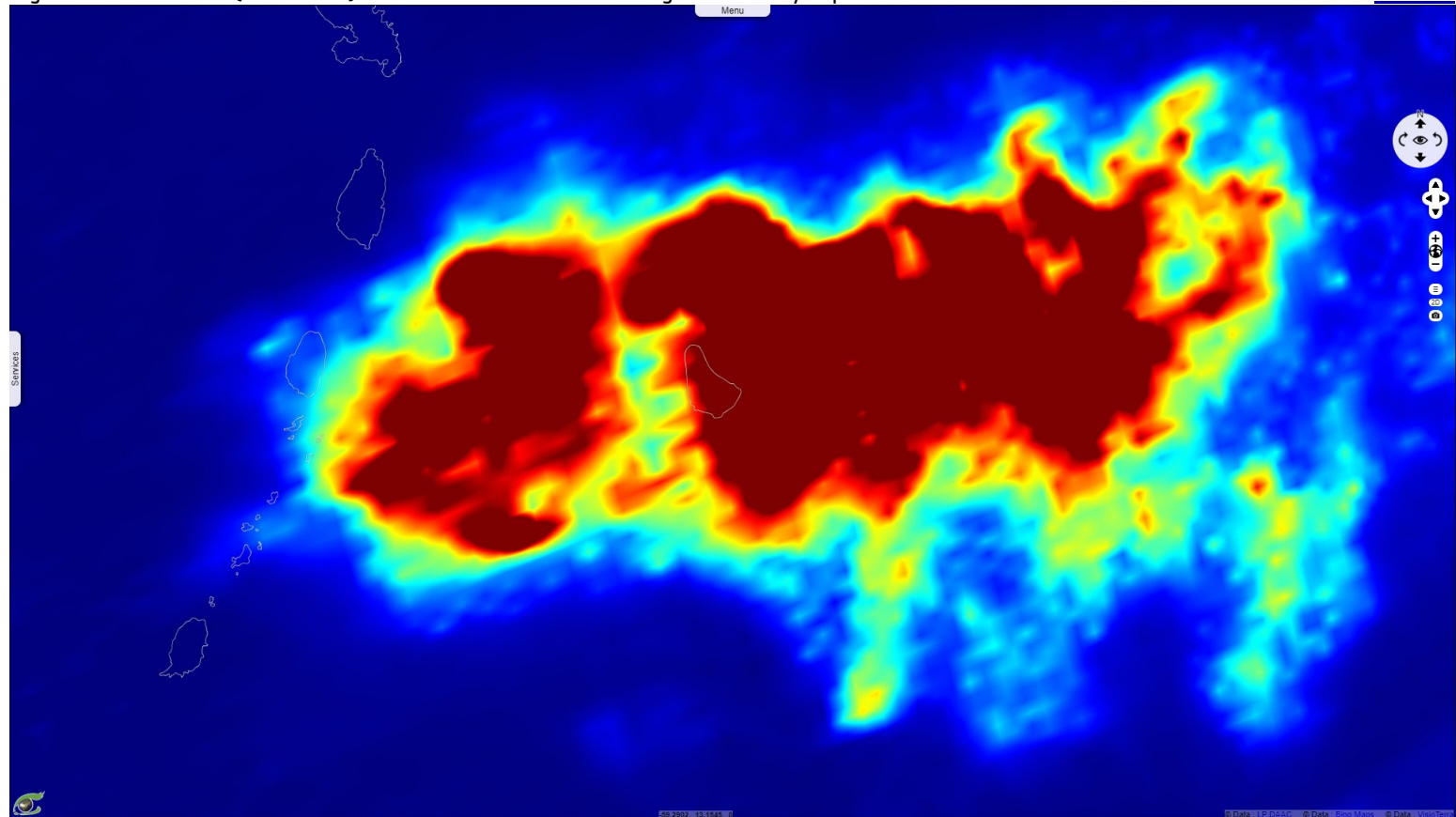
Fig. 3 - S2 (03.01.2020) - View last year before the current eruption.
