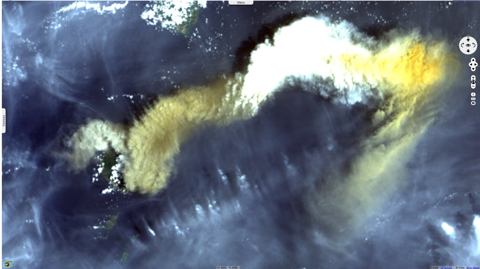
Fig. 1 - S3 OLCI (09.04.2021) - La Soufrière volcano has been active since Decembre, its eruption is scaling up.
