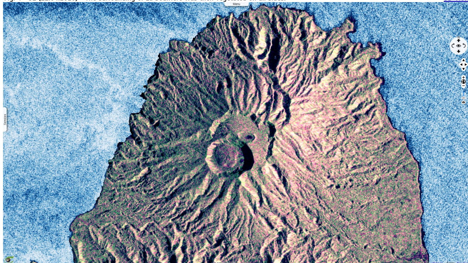
Fig. 5 - S1 (12.04.2021) - The crater had its domes have changed significantly, southern and western valleys as well.
