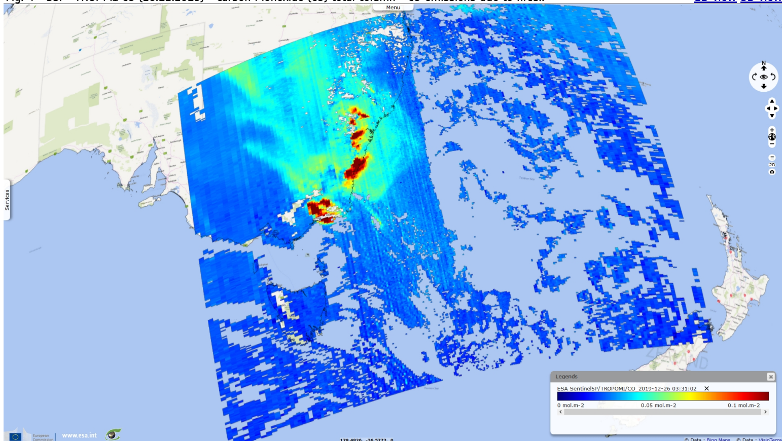
Fig. 4 - S5P- TROPOMI CO (26.12.2019) - Carbon Monoxide (CO) total column - CO emissions due to fires..
