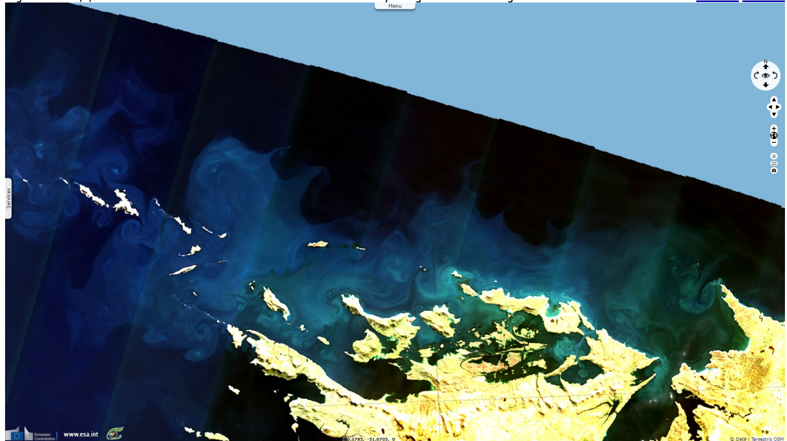
Fig. 4 - S2 - 4,3,2 natural colour - Plankton colours and concentration vary along this 200-km long bloom. 3D view 2D view
