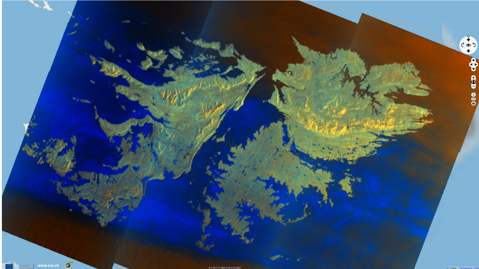
Fig. 2 - S2 (18 & 20.04.2018) - 11,8,2 colour composite - View of the isthmus of East Falkand, the archipelago's largest island.
