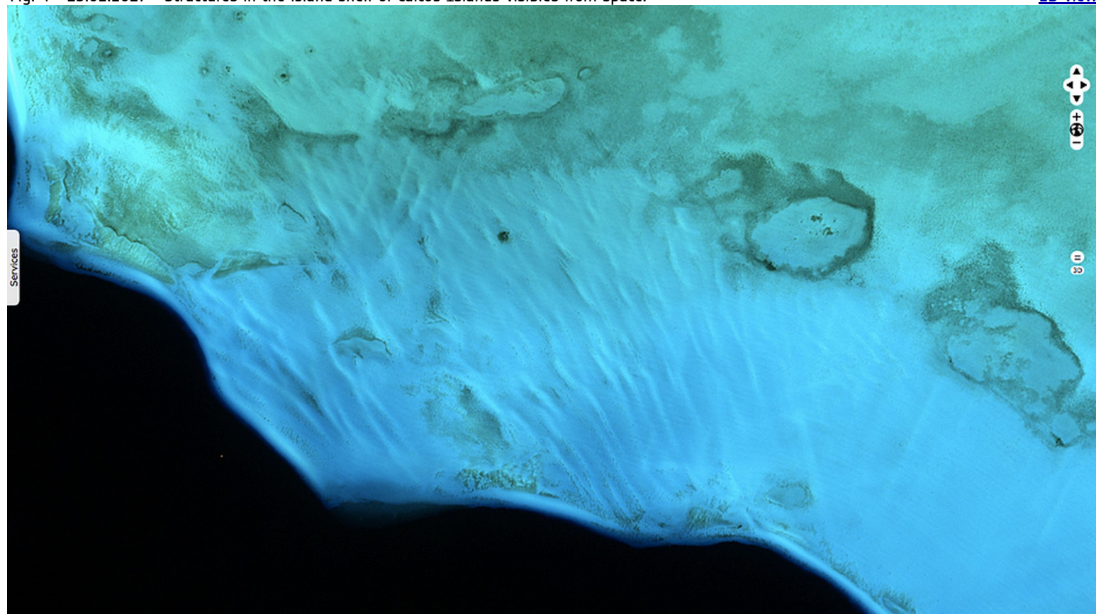
Fig. 4 - 13.02.2017 - Structures in the island shelf of Caicos Islands visibles from space.
