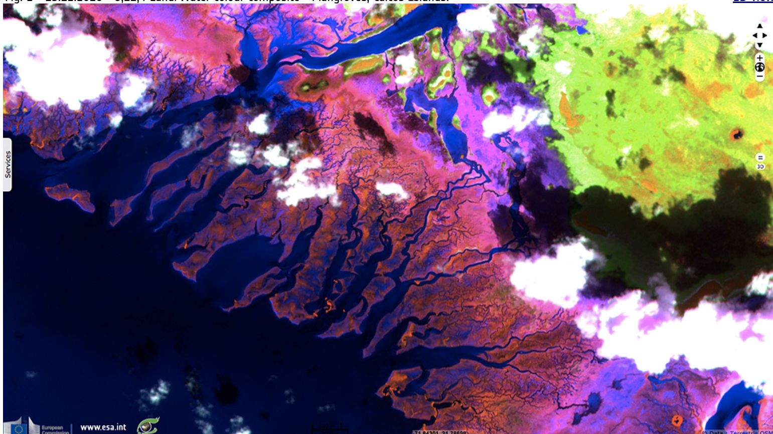
Fig. 2 - 15.12.2016 - 8,11,4 Land/Water colour composite - Mangroves, Caicos Islands.
