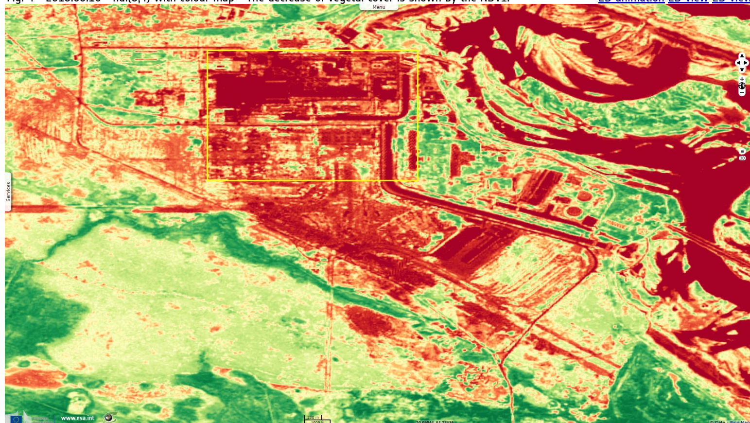
Fig. 4 - 2018.06.10 - ndi(8,4) with colour map - The decrease of vegetal cover is shown by the NDVI. 2D animation 2D view 2D view
