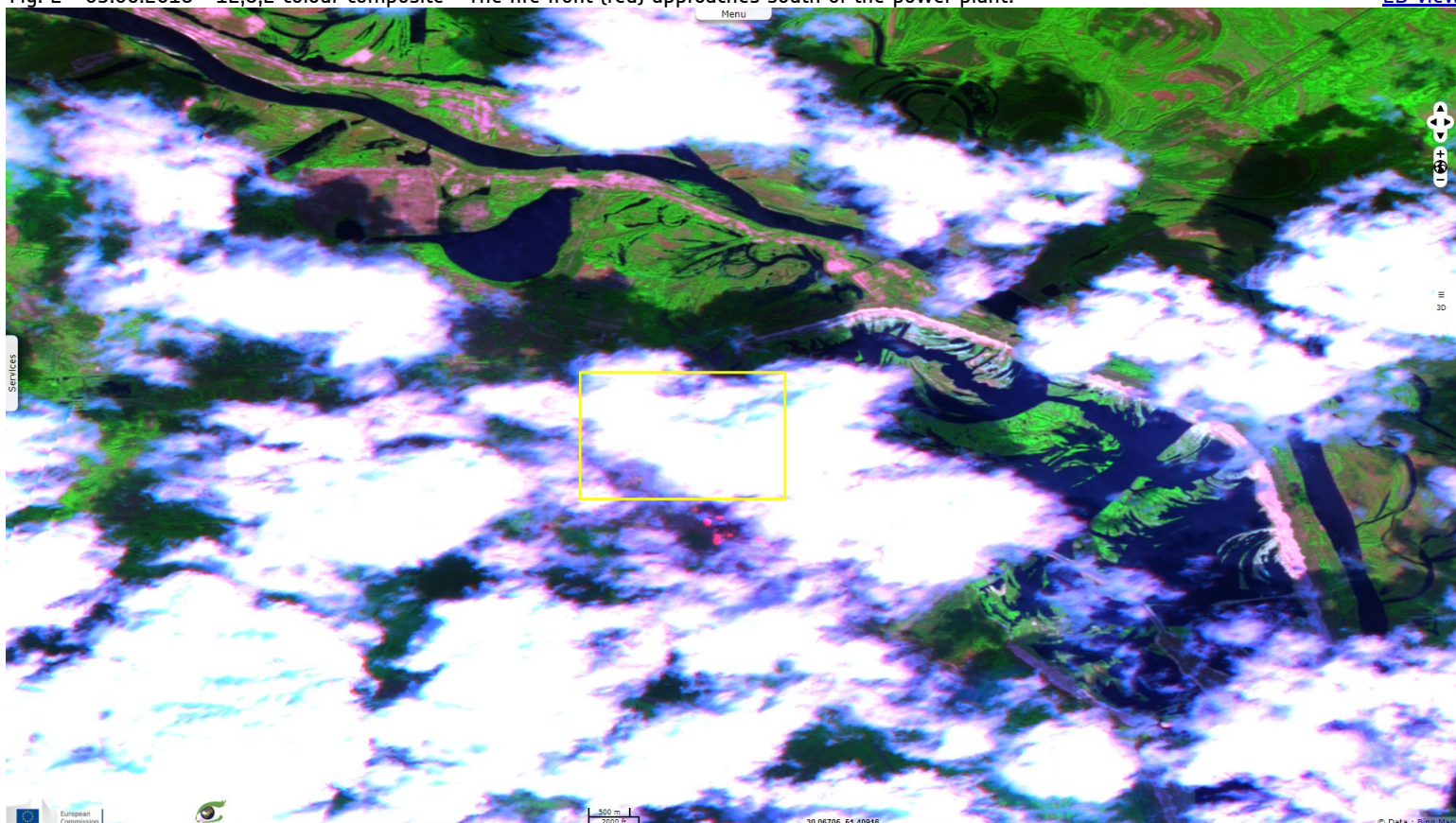
Fig. 2 - 05.06.2018 - 12,8,2 colour composite - The fire front (red) approaches south of the power plant.
