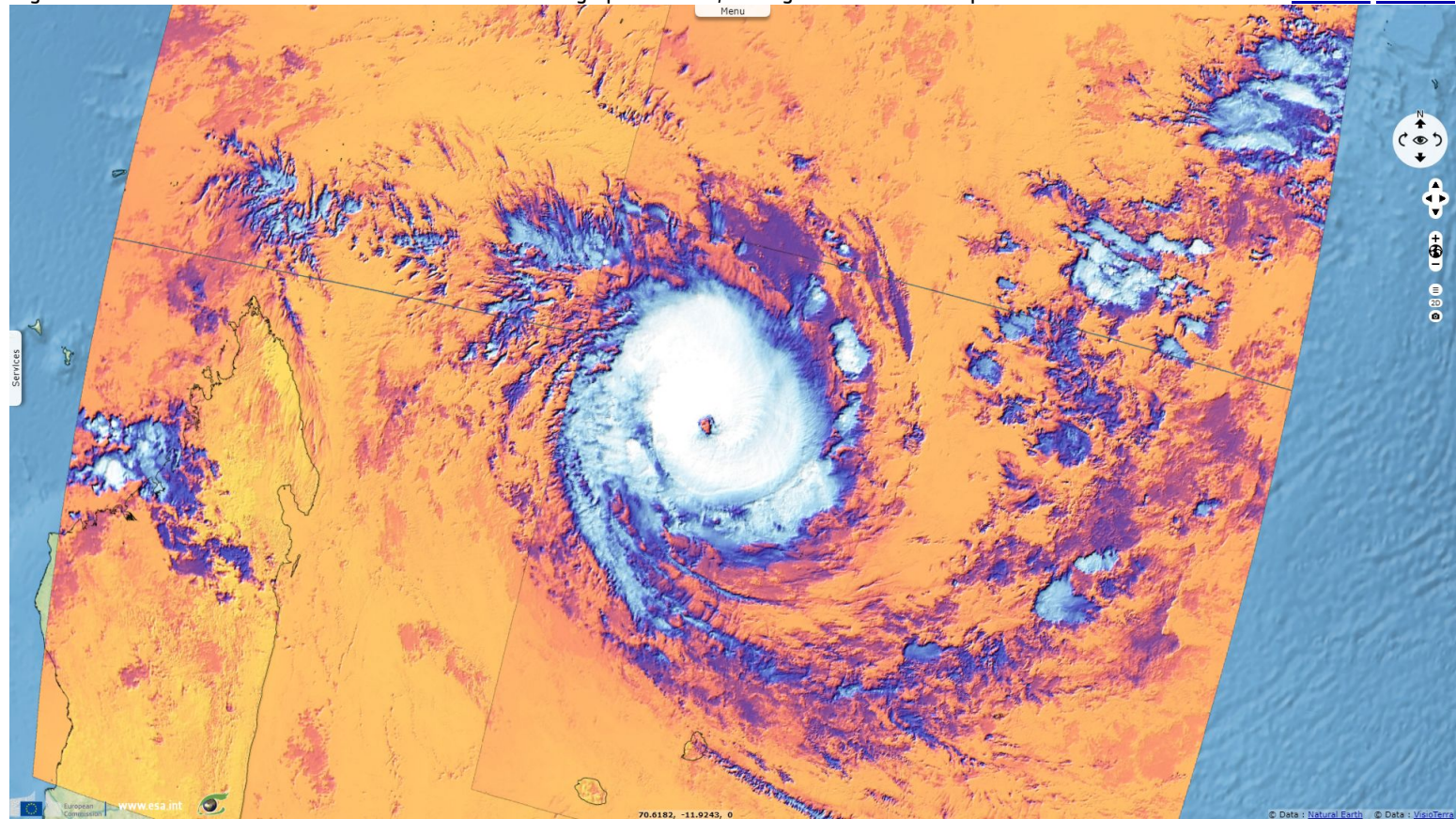
Fig. 3 - S3B & S3A SLSTR - S8 thermal band - For such huge phenomena, adding both near-contemporaneous swaths is useful. 2D view 3D view
