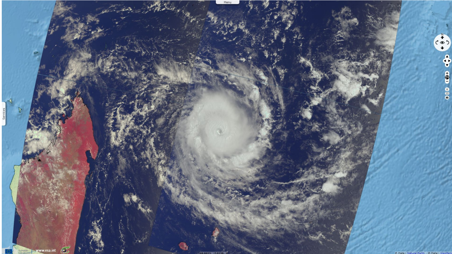
Fig. 2 - S3B & S3A SLSTR - S6,S5,S2 colour composite - It was viewed by S3B (east) & S3A (west) 40mn apart.
