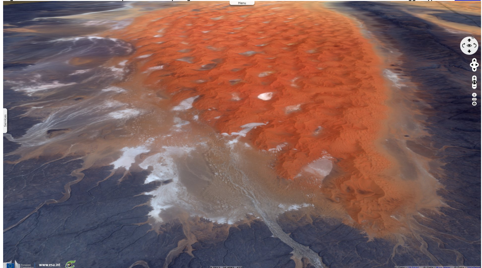
Fig. 4 - Mesoscale dunes move slowly over stationary megadunes while smaller dunes form & move faster over the backs of bigger types. 3D view
