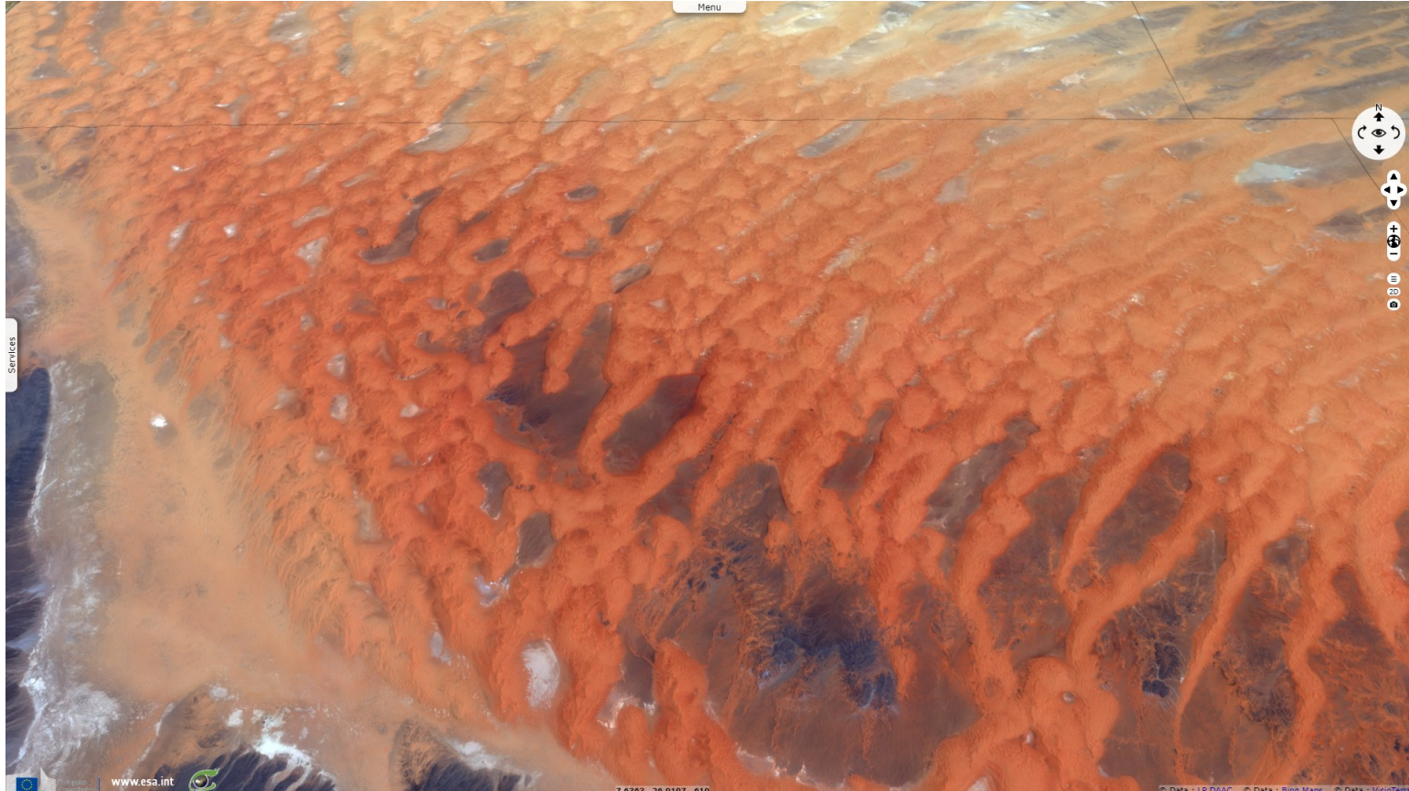
Fig. 2 - S2 (30.05.2020) - Dune corridors arrangement over the darker flat floor at S-E of Erg Issaouane. Some enclose sabkhahs, or salt flats. 2D view
