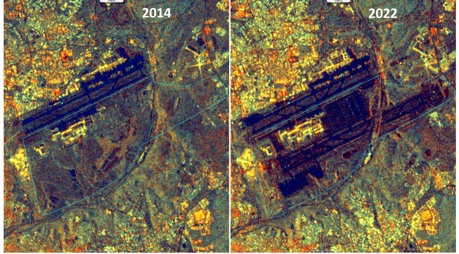
Fig. 4 - S1 (09.10.2014->02.11.2014 / 12->24.01.2022) - Sabiha Gökçen Airport, a 2nd runway was built in 2022. 3D view 3D view
