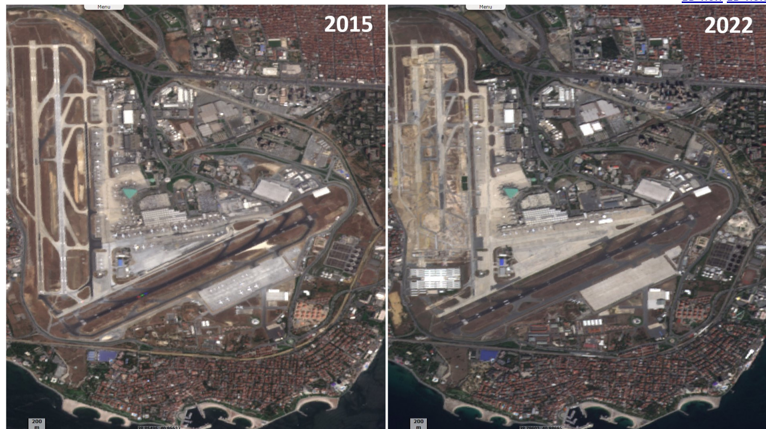
Fig. 3 - S2 (12.08.2015 / 01.10.2022) - Atatürk Airport was closed to passengers in 2019, to freight in Feb. 2022, demolition works began in May 2022.
