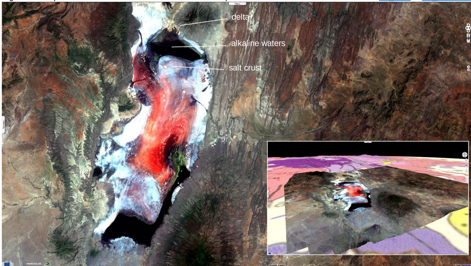
Fig. 2 - S2 acquired on 08.02.2017 - 4-3-2 Natural colour composite
