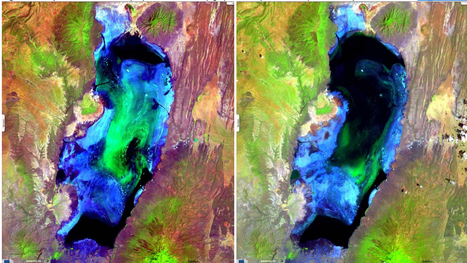
Fig. 4 - S2 acquired on 20.12.2016 (left) v.s. 08.02.2017 (right) - (B7-B5) red edge normalised difference
