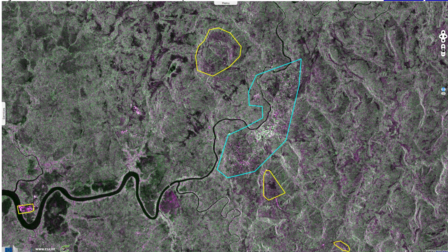
Fig. 2 - S1 (21.01.2018) - vv,vh,vv colour composite - Developpt of bauxite mines near Boke in Korinko, Fotonkoneya & Kakoui.
