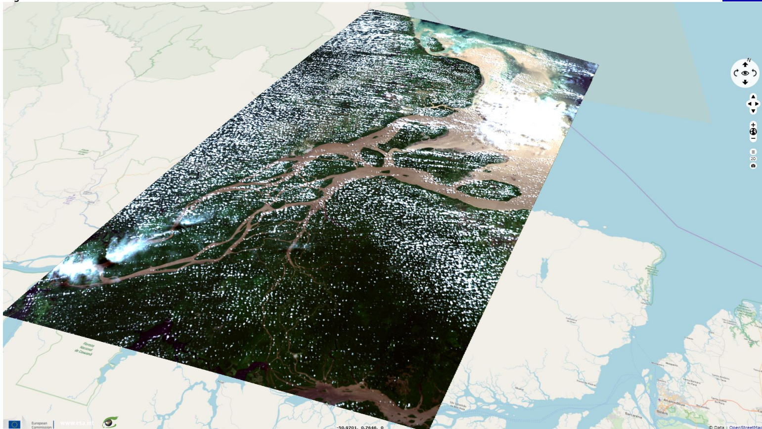
Fig. 2 - 4-3-2 natural colour - Alluvium filled Amazon waters enter the 50km wide river mouth.
