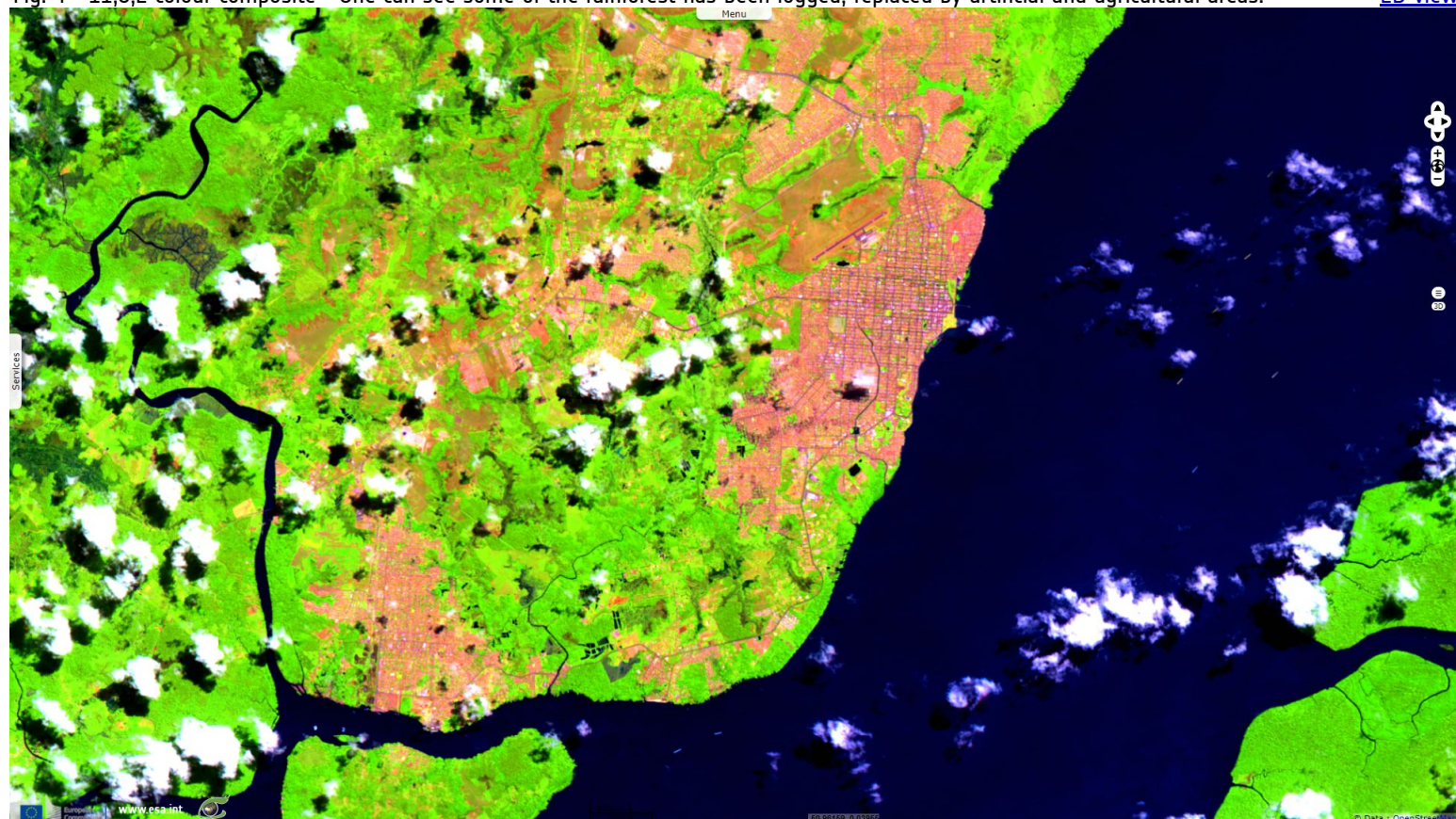
Fig. 4 - 11,8,2 colour composite - One can see some of the rainforest has been logged, replaced by artificial and agricultural areas.
