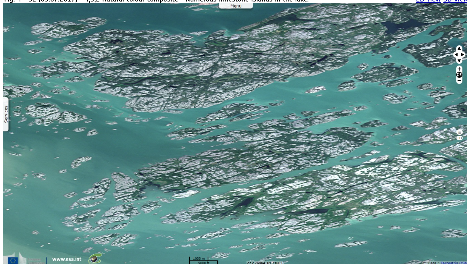
Fig. 4 - S2 (09.07.2017) - 4,3,2 Natural colour composite - Numerous limestone islands in the lake.
