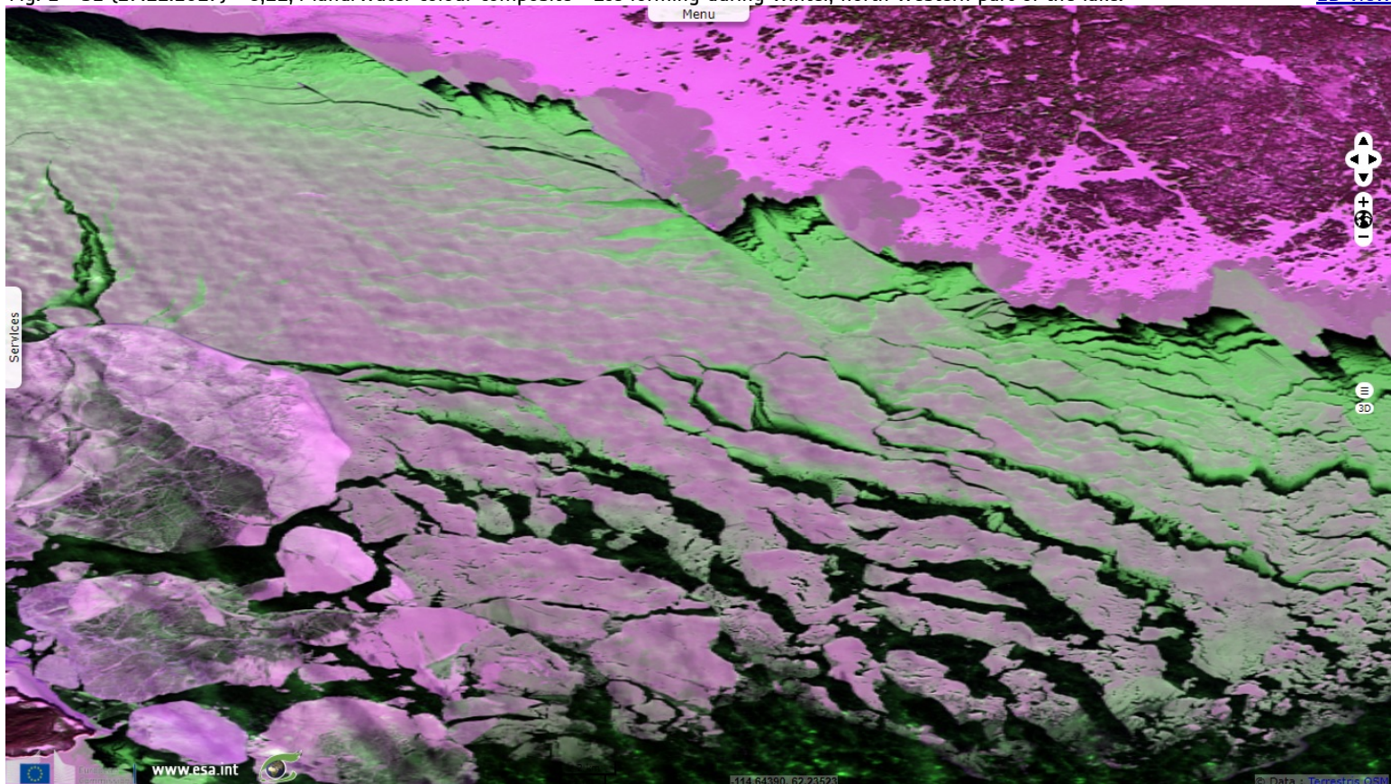
Fig. 2 - S2 (17.11.2017) - 8,11,4 land/water colour composite - Ice forming during winter, north western part of the lake.
