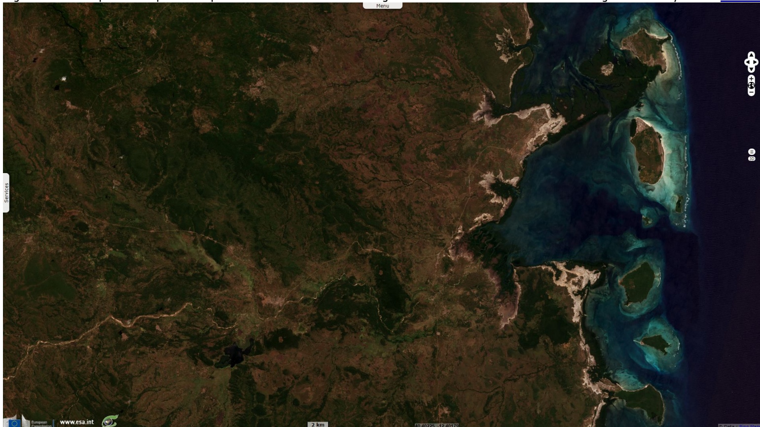
Fig. 2 - A national park encompasses its pristine sand bars & coral reefs together with mainland features such as mangrove-filled bays.
