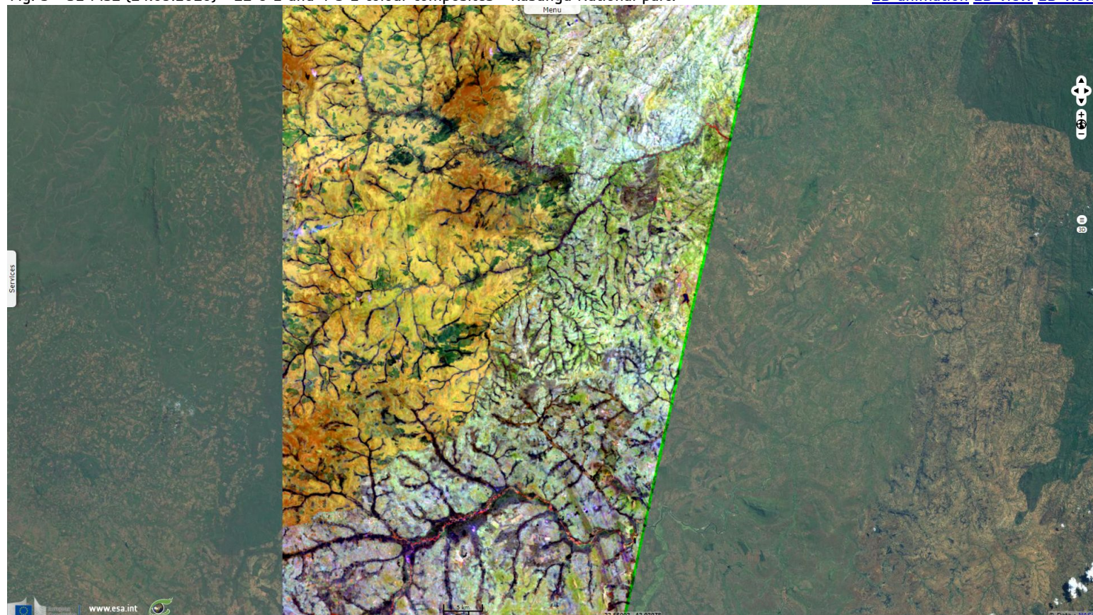
Fig. 4 - S2 MSI (22.08.2016) - 4-3-2 natural colour - Part of the huge rift Lake Malawi (also called Niassa) seen from its west bank. 3D view 2D view
