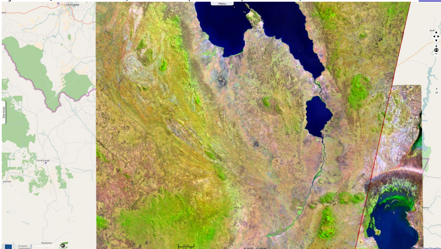
Fig. 2 - S2 MSI (22.08.2016 & 09.08.2016) - 4-3-2 natural colour - Water colour change from one lake to the next.
