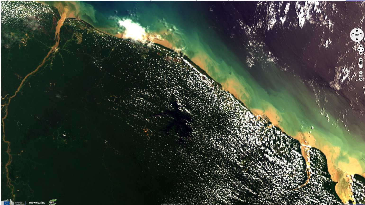
Fig. 2 - OLCI (14.08.2018) - 10,6,3 natural colour - French Guyana is delimited by Moroni & Oyapock rivers.
