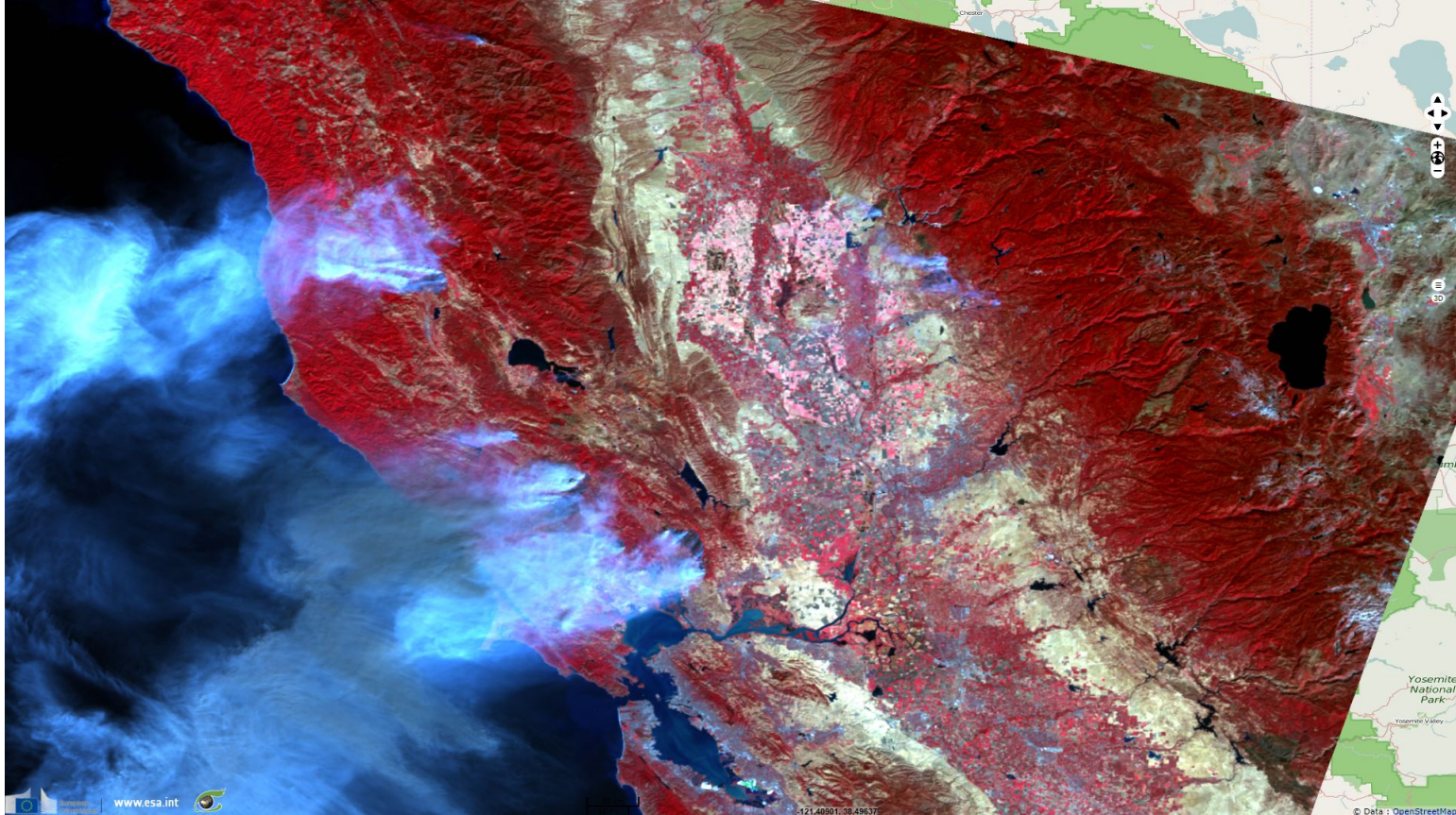
Fig. 2 - SLSTR (09.10.2017 & 10.10.2017) - S6,S3,S2 composite - Active fronts show in red, burnt areas in brown. 2D view 2D view 2D animation
