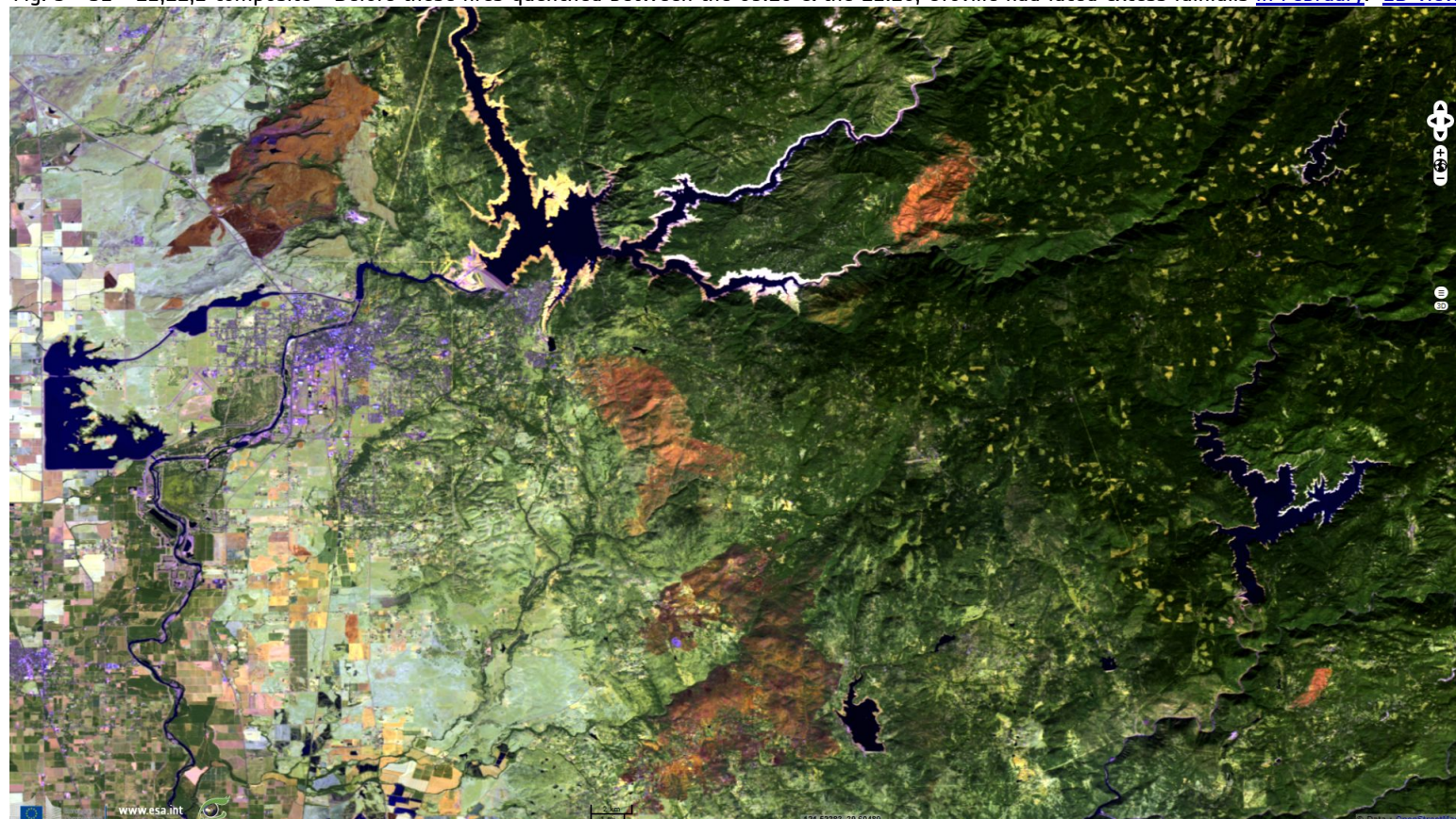
Fig. 4 - S2 - 12,8,3 composite - Active wildfires near Napa urban areas that killed over thirty and destroyed thousands homes. 2D view
